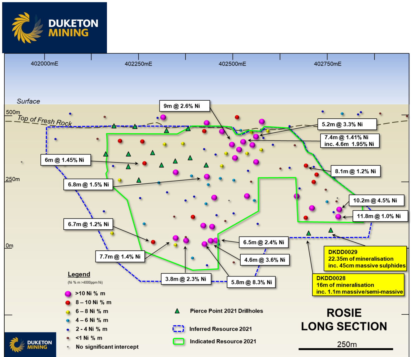
Figure 5: Long Section of Rosie showing pierce points of 2021 drillholes
