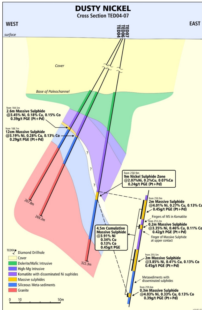
Figure 5: E-W cross-section through diamond drill holes TED04, TED06 and TED07 at Dusty 1. Note that TED11 has not be added to this cross-section. The nickel sulphide intersection in TED11, not shown here, is approximately 20m down-dip to the east of TED07.
