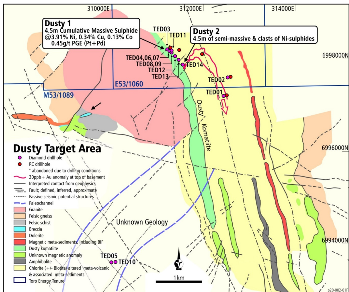
Figure 3: Location of TED14 relative the original Dusty Nickel Discovery within the Dusty Target Area.
