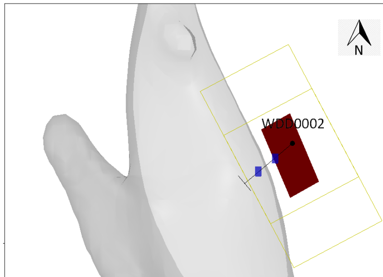
Figure 4: Plan view of conductor plate (red) beneath the 21WDD0002 hole trace. Highly magnetic body beneath conductor in grey, DHEM surface loops in yellow
