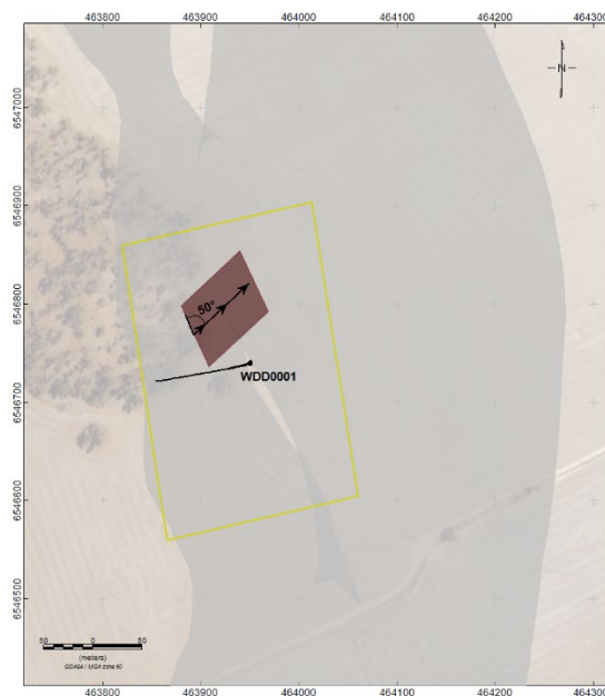
Figure 5: Plan view of plate 20a showing location of conductor plates and hole 21WDD0001 trace
