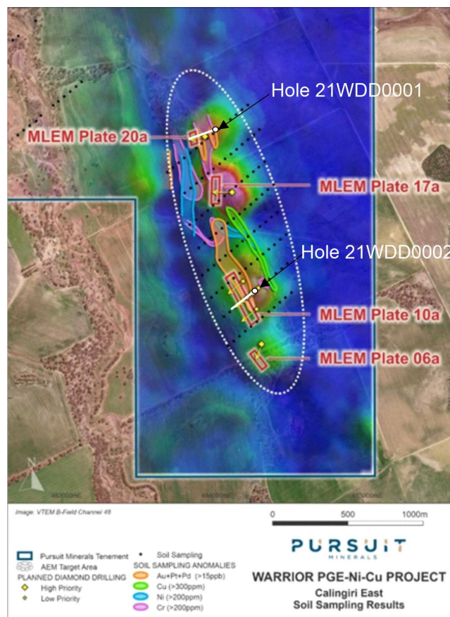
Figure 1: Phil’s Hill EM target plates, surface geochemistry and completed drillholes
