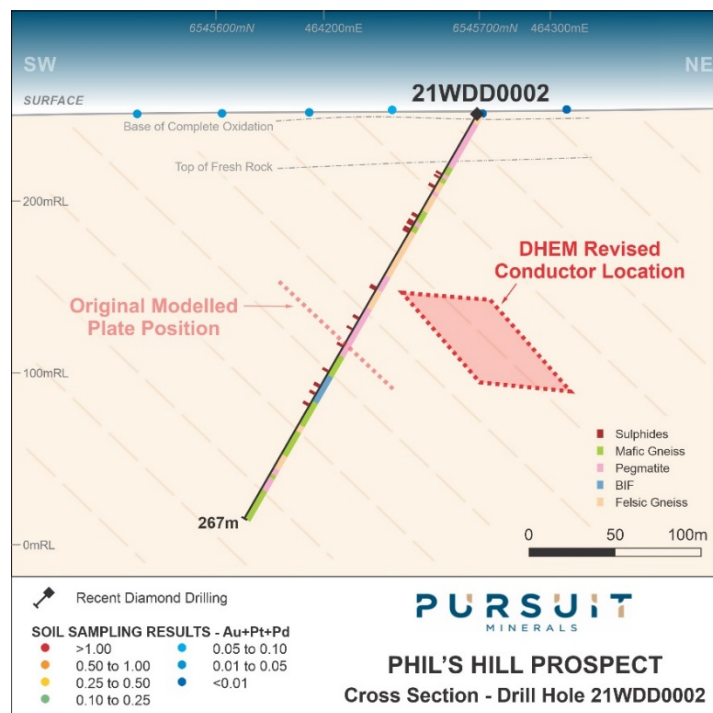
Figure 3: Schematic Cross section through strongest conductor Plate 10a showing revised conductor position
