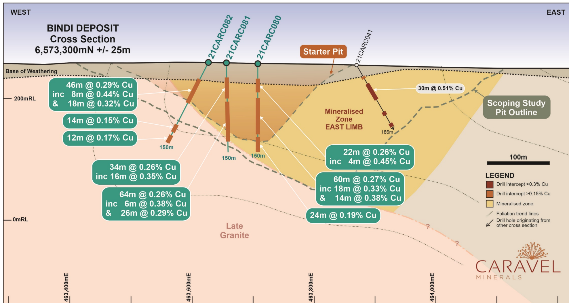
Figure 3: Schematic geological cross section of the Bindi Deposit (6,573,300mN) showing location of recent RC percussion (CARC prefix) diamond core (CADD prefix) and diamond tail (CADT prefix) drill holes and mineralised intersections.
