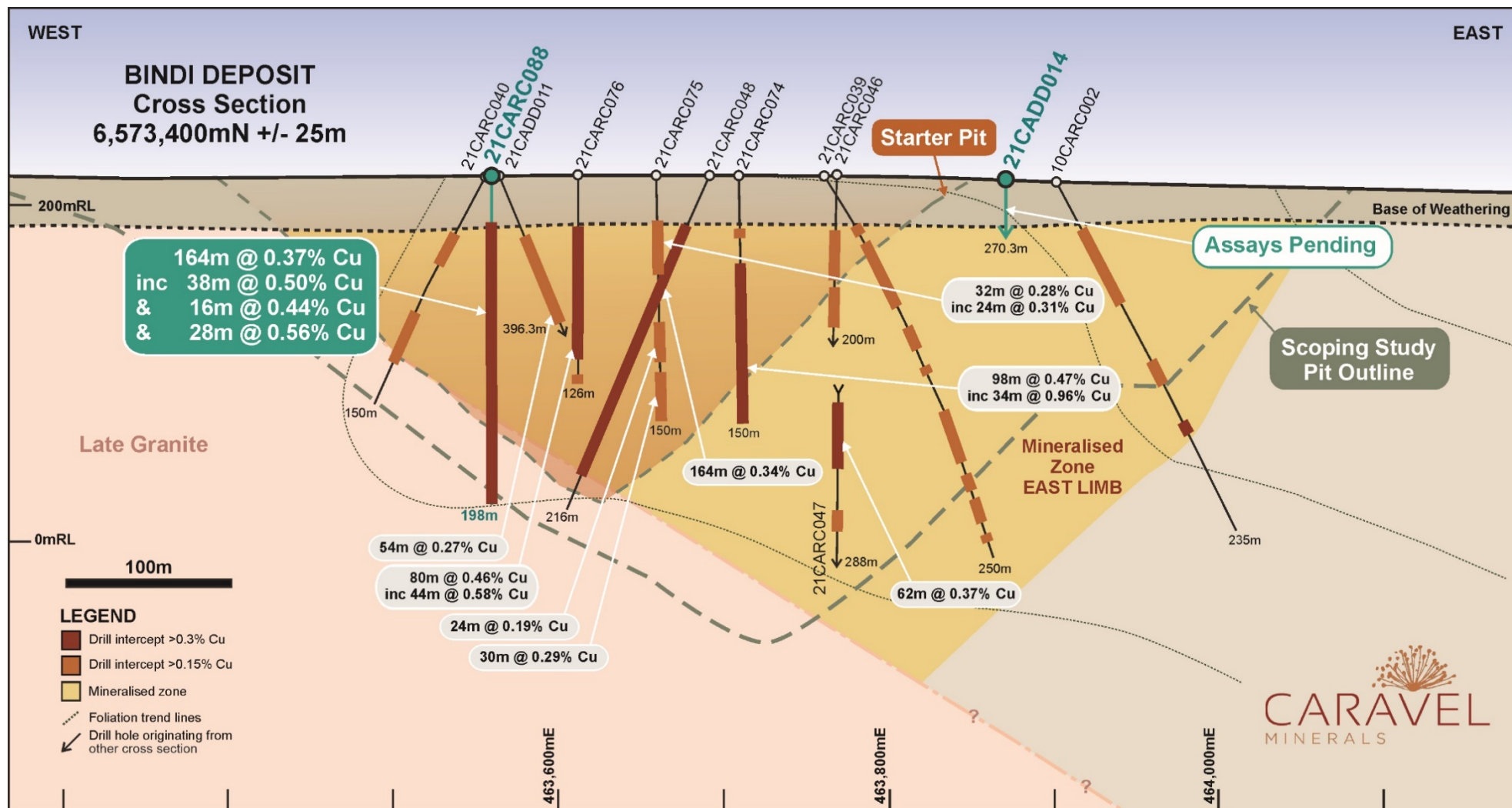
Figure 5: Schematic geological cross section of the Bindi Deposit (6,573,400mN) showing location of recent RC percussion (CARC prefix) diamond core (CADD prefix) and diamond tail (CADD prefix) drill holes and mineralised intersections.
