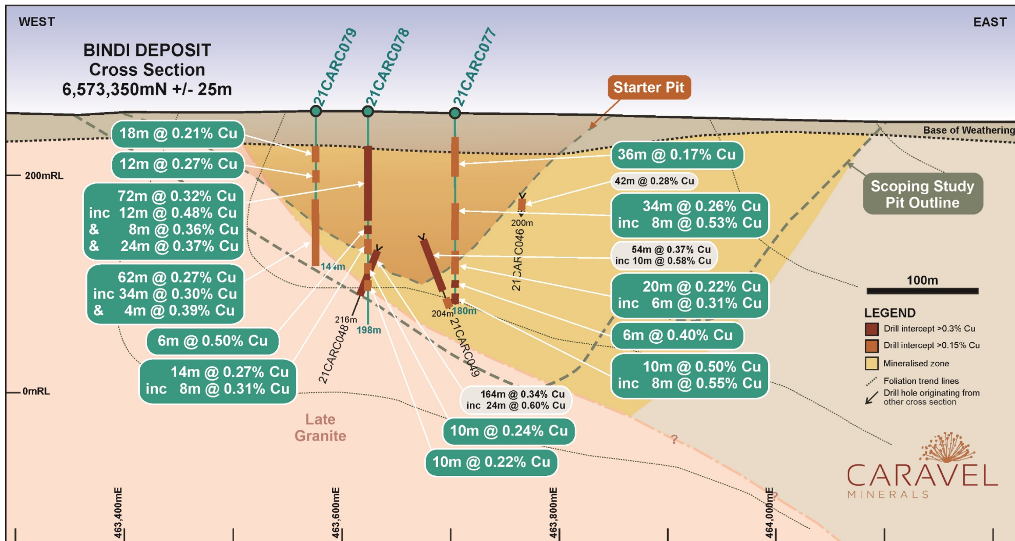
Figure 4: Schematic geological cross section of the Bindi Deposit (6,573,350mN) showing location of recent RC percussion (CARC prefix) diamond core (CADD prefix) and diamond tail (CADT prefix) drill holes and mineralised intersections.
