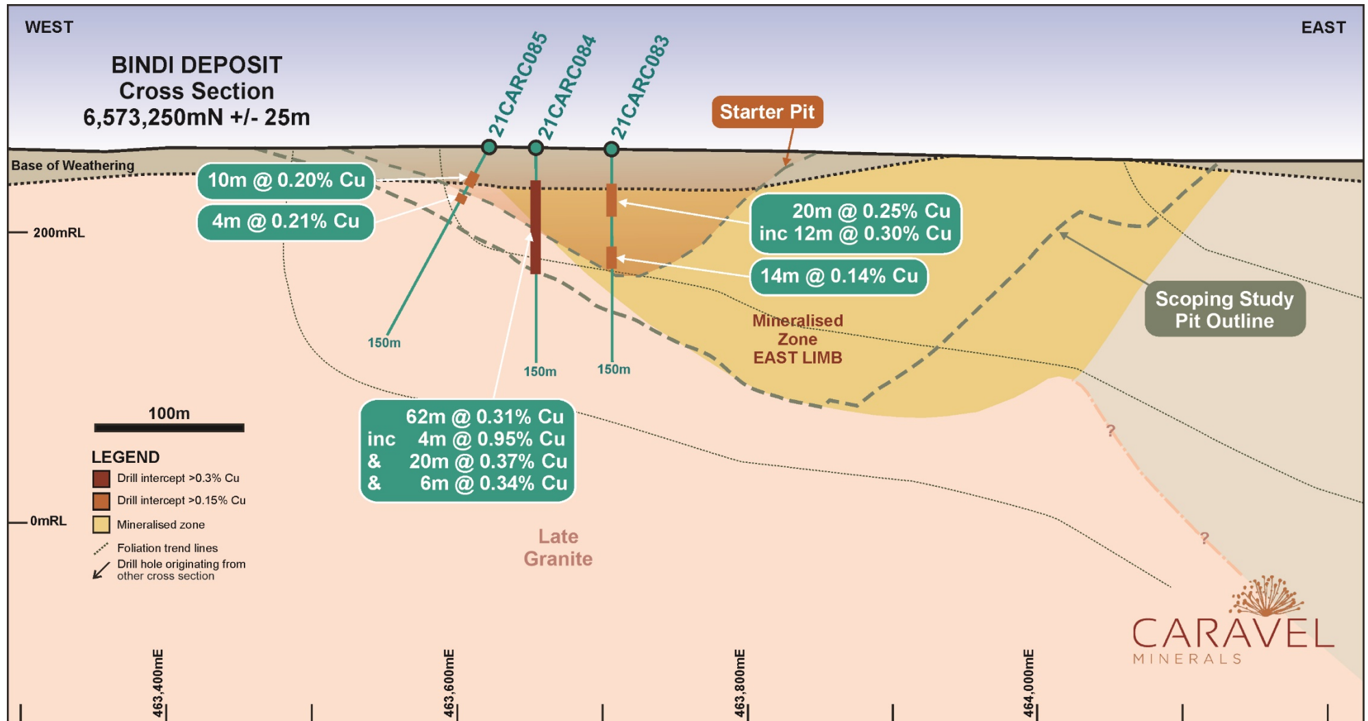
Figure 2: Schematic geological cross section of the Bindi Deposit (6,573,250mN) showing location of recent RC percussion (CARC prefix) diamond core (CADD prefix) and diamond tail (CADT prefix) drill holes and mineralised intersections.
