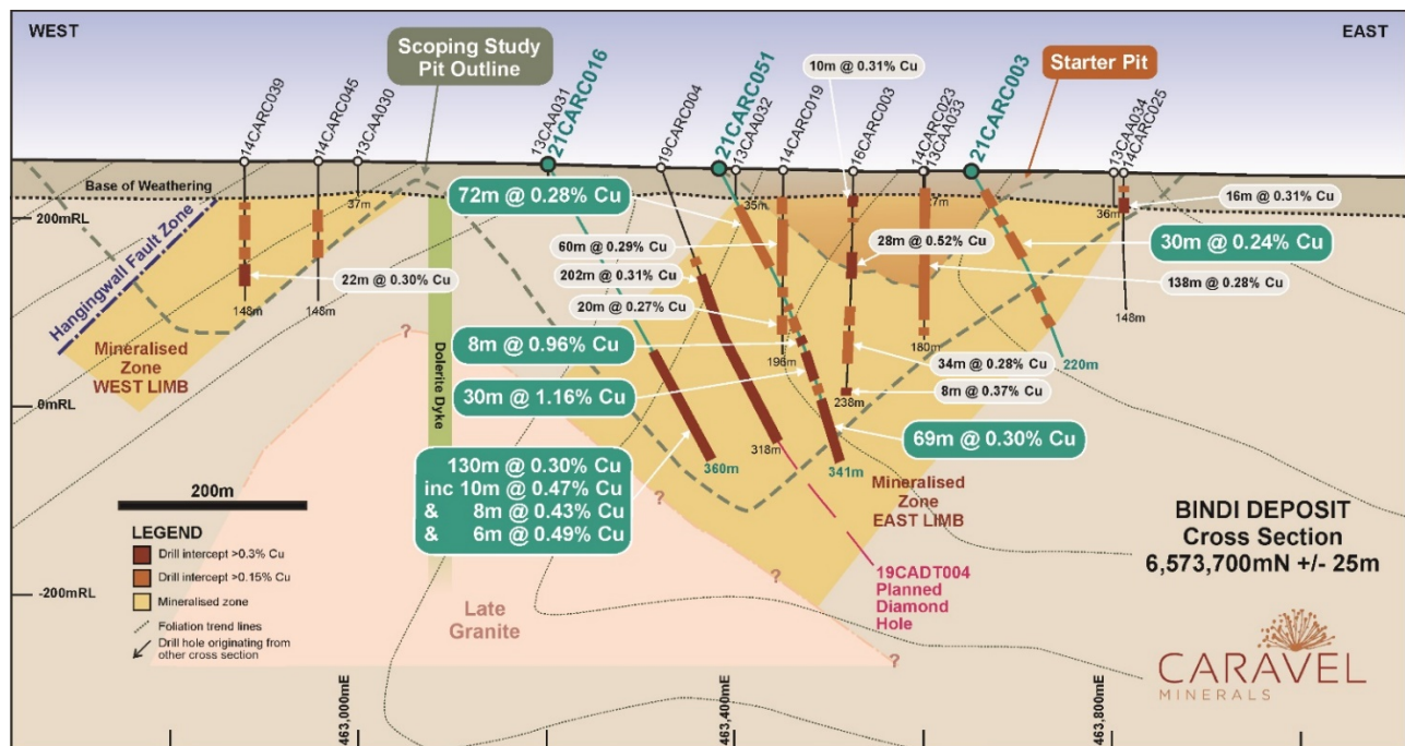
Figure 9: Schematic geological cross section of the Bindi Deposit (6,573,700mN) showing location of recent RC percussion (CARC prefix) diamond core (CADD prefix) and diamond tail (CADT prefix) drill holes and mineralised intersections.
