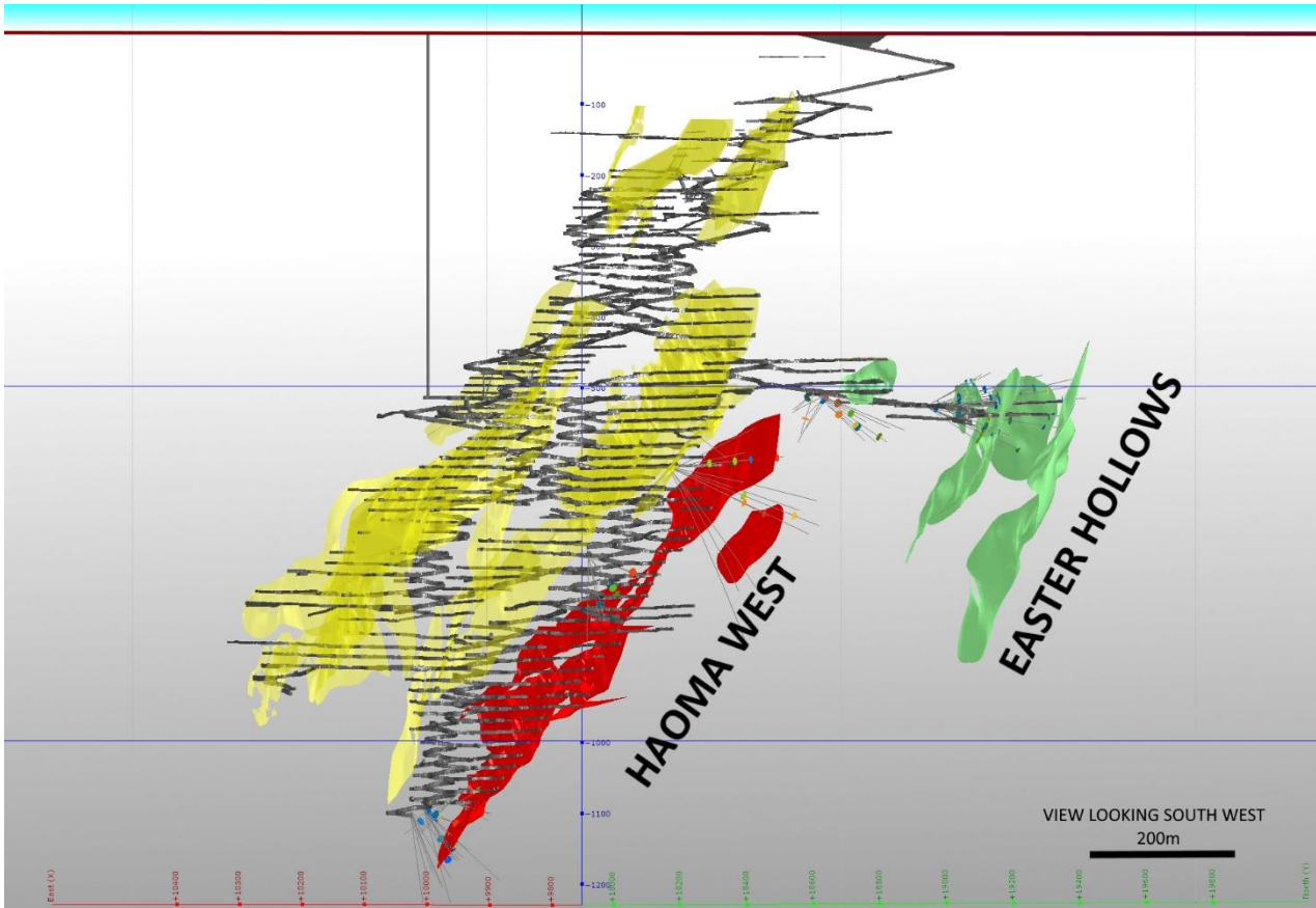
Figure 11: Daisy Complex highlighting established underground development and Easter Hollows zone
