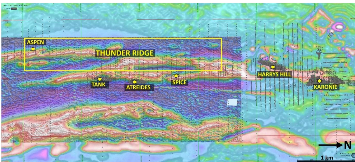
Figure 13 Regional Aldiss magnetic survey, highlighting Thunder Ridge trend and Aspen relative to SAT trend deposits
