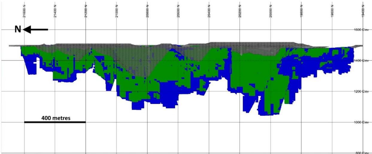
Figure 12: Long section view (looking east) of the Santa Mineral Resource block model showing Indicated Resources (green) and Inferred Resources (blue). The optimised open pit shell is shown in grey
