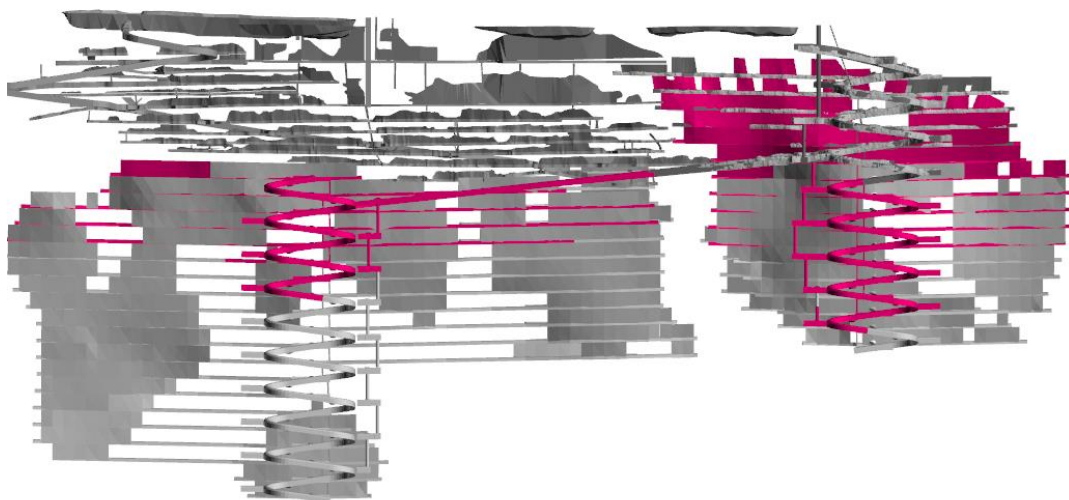
Figure 5: Rothsay long section showing FY22 mine schedule (magenta) v LOM design (looking east)
