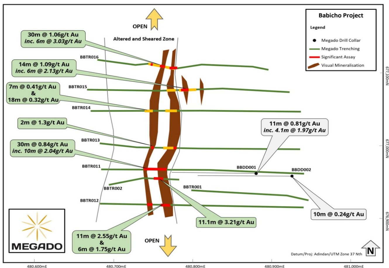
Figure 1 – Phase 2 trenching results at the Babicho Gold Project
