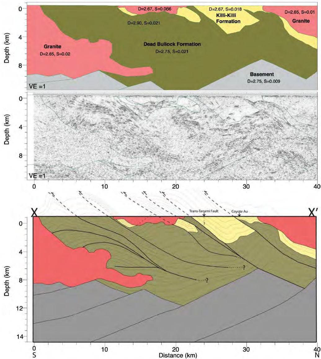
Figure 11: Profile X-X': 2D joint (gravity and magnetic) forward model, 6s migrated section of seismic profile 05GA-T2.
