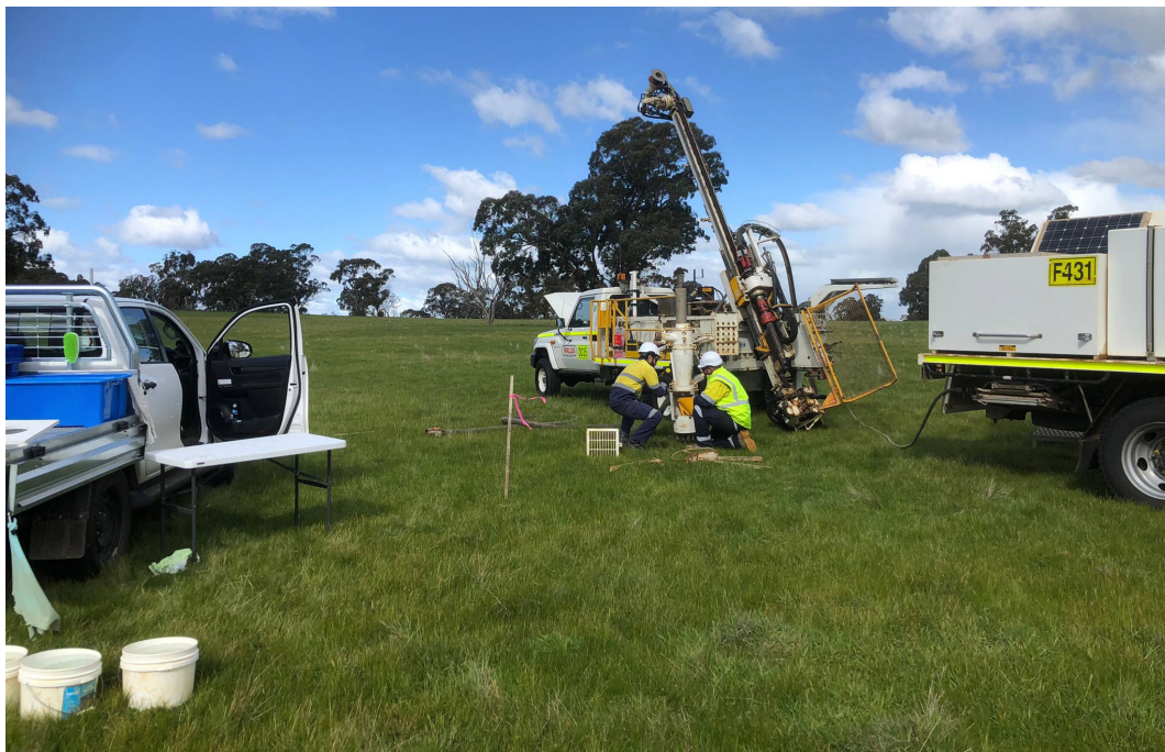
Figure 1: Wallis Drilling Mantis Aircore Rig in Action
