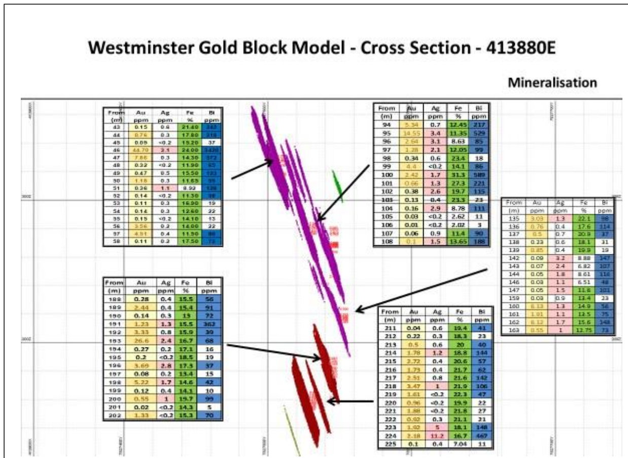
Figure Twelve: Ore Body – Model Slice – Polymetallic Mineralisation
