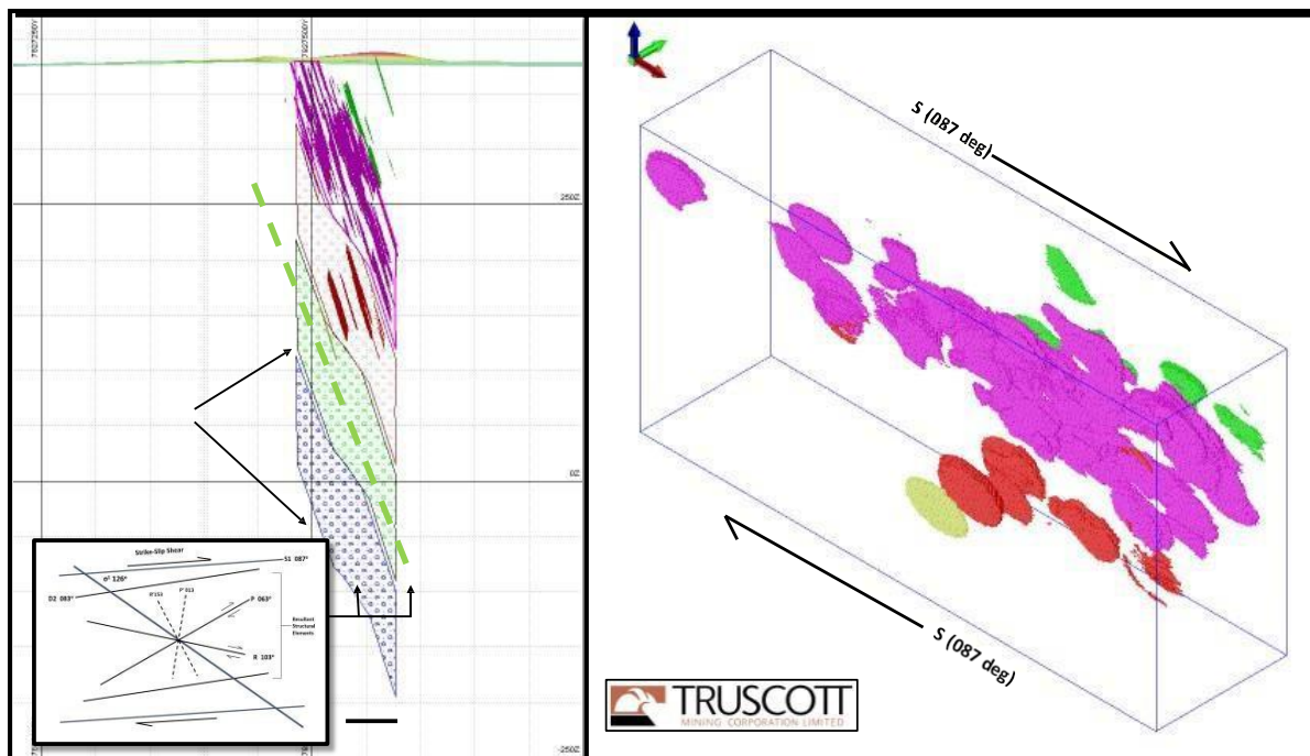
Figure Ten: Modelling Mineralising fluid flows and Dilation Shear Interaction – Westminster Project
