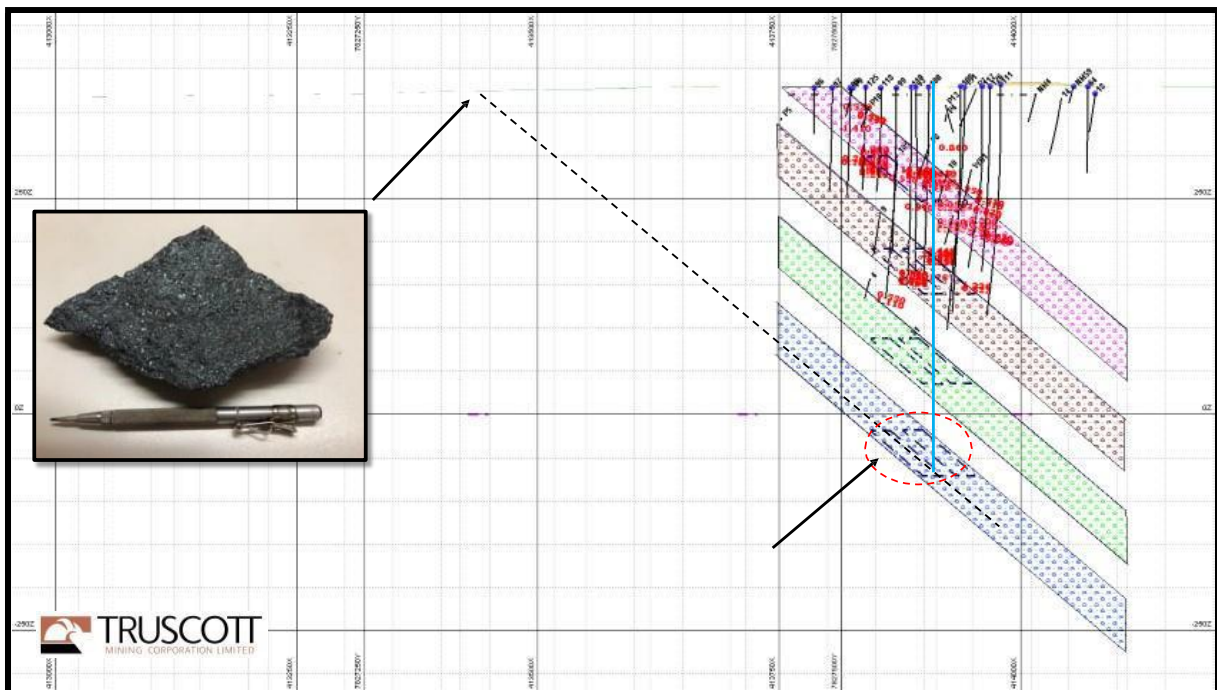
Figure Eleven: Westminster Project – Drill Section 1.6
