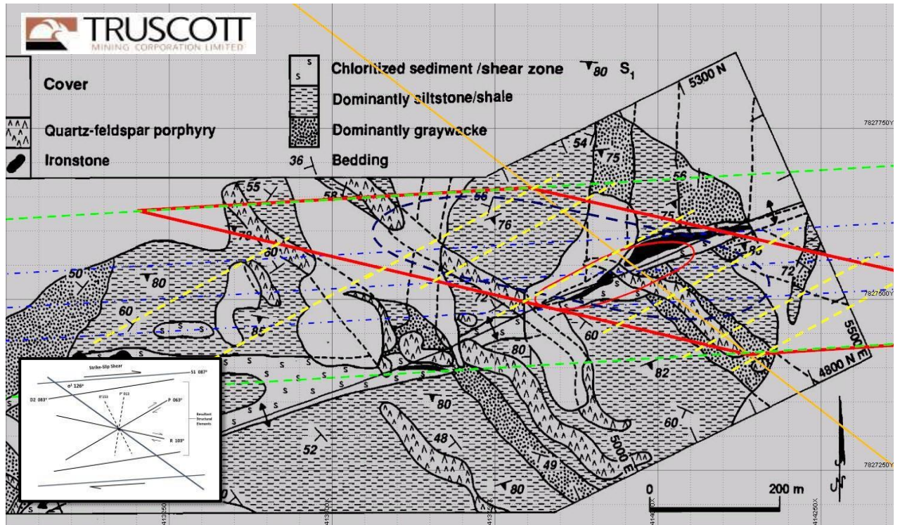
Figure Seven: Observations at Ore Body Level (Fractal Four) White Devil Deposit – Ore Body Alignment
