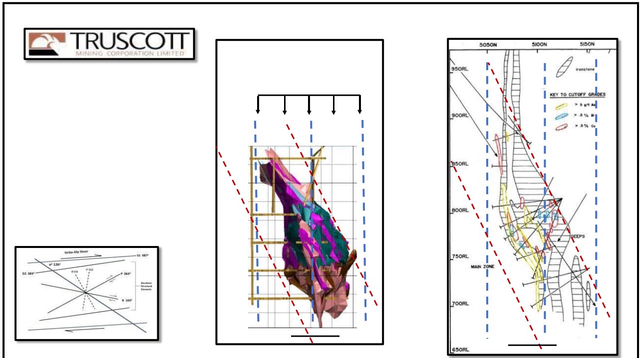
Figure Eight: Interactions of Mineralising Fluids and Dilation – Juno & White Devil Deposits
