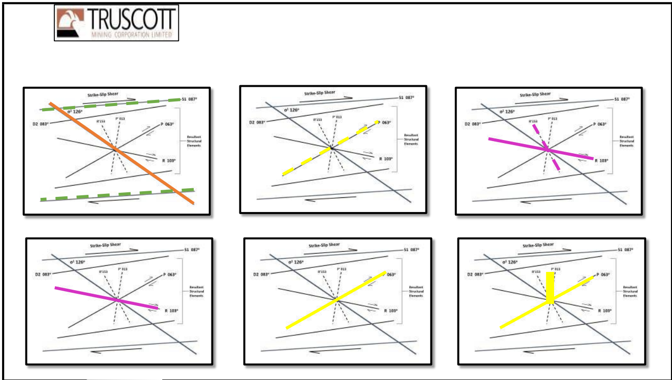
Figure Fourteen: Confirming Remote Analysis of Strike-slip Shear elements with Field Observations
