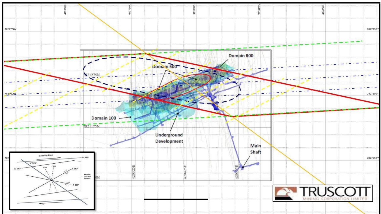
Figure Six: Observations at Ore Body Level (Fractal Four) Juno Deposit – Ore Body Block Model
