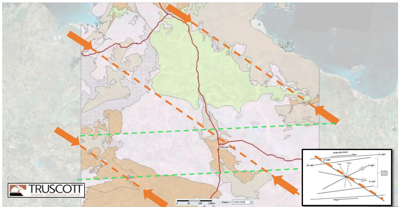
Figure Two: Regional Linear observations on 126^\circ (Sigma 1)
