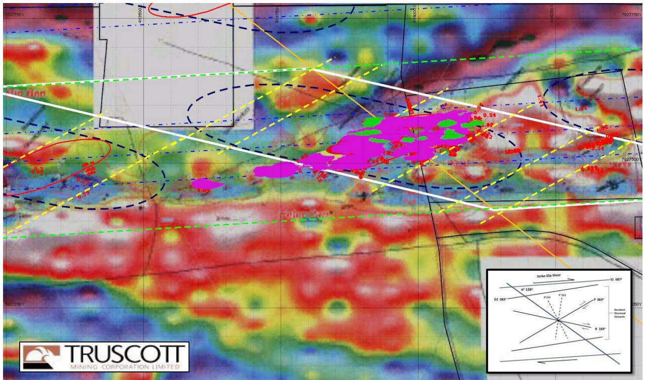
Figure Nine: Ore Body Level (Fractal Four) Westminster – Gold Block Model & Gravity Image
