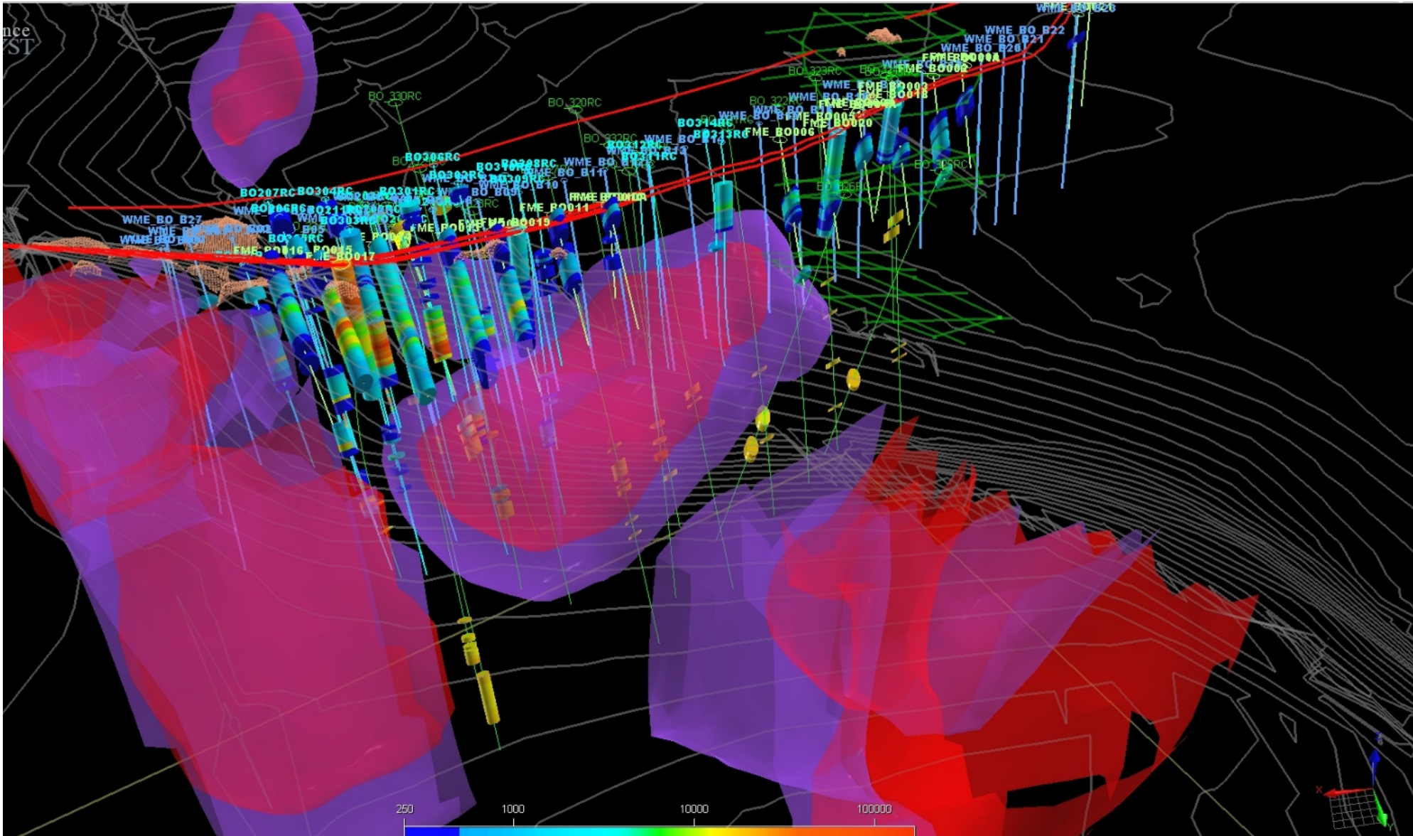
FIGURE A1-2: 3D VIEW OF IP ANOMALIES AND DRILLHOLES COPPER ASSAY >250PPM, LOOKING SOUTH-SOUTHWEST
