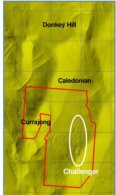
Figure 1 Adelong deposits
