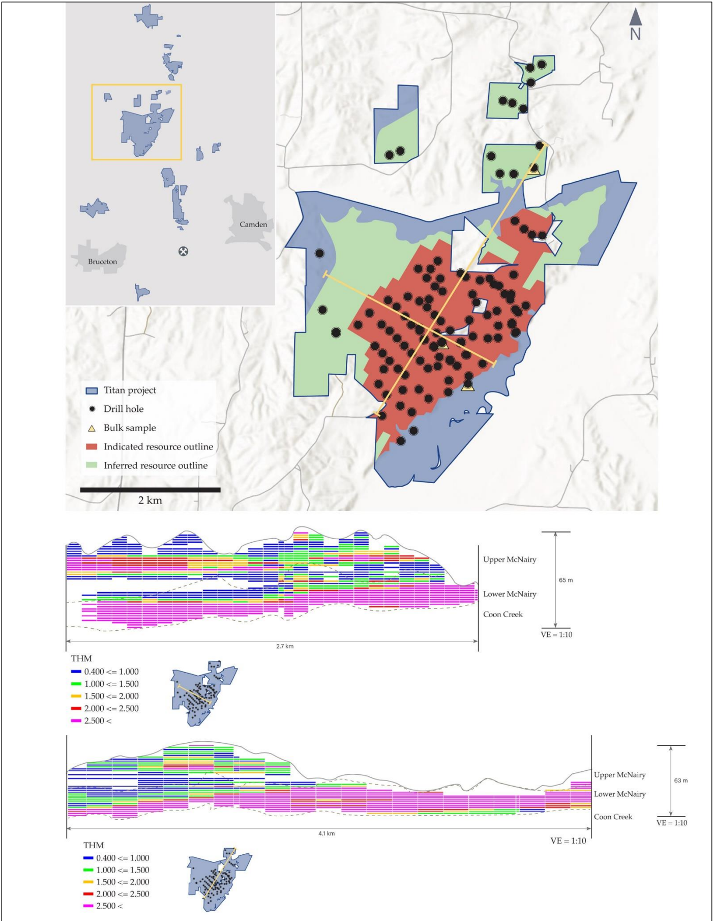
Figure 8: MRE plan view, cross section and long section.
