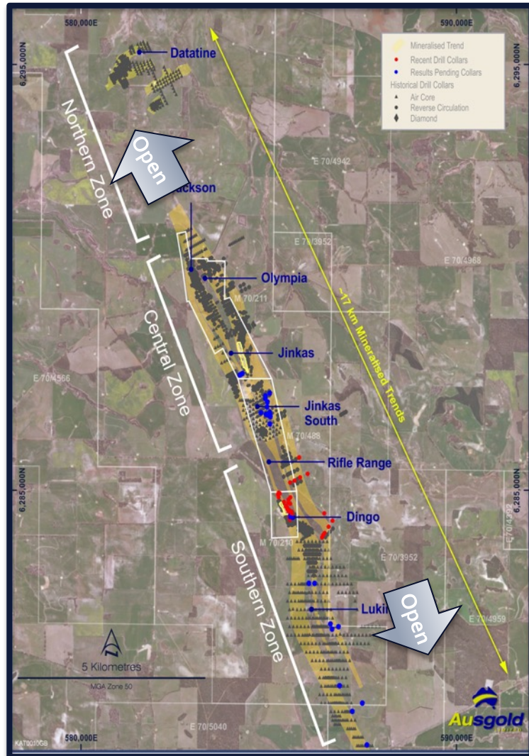
Katanning - Main Strike Zone Areas
