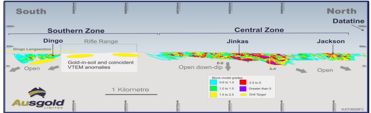
Katanning Long section highlighting the Central Zone
