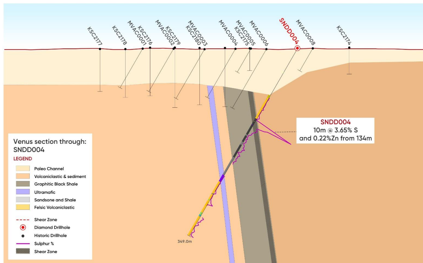
Figure 5. Schematic section of drilling (SNDD004) completed at Venus
