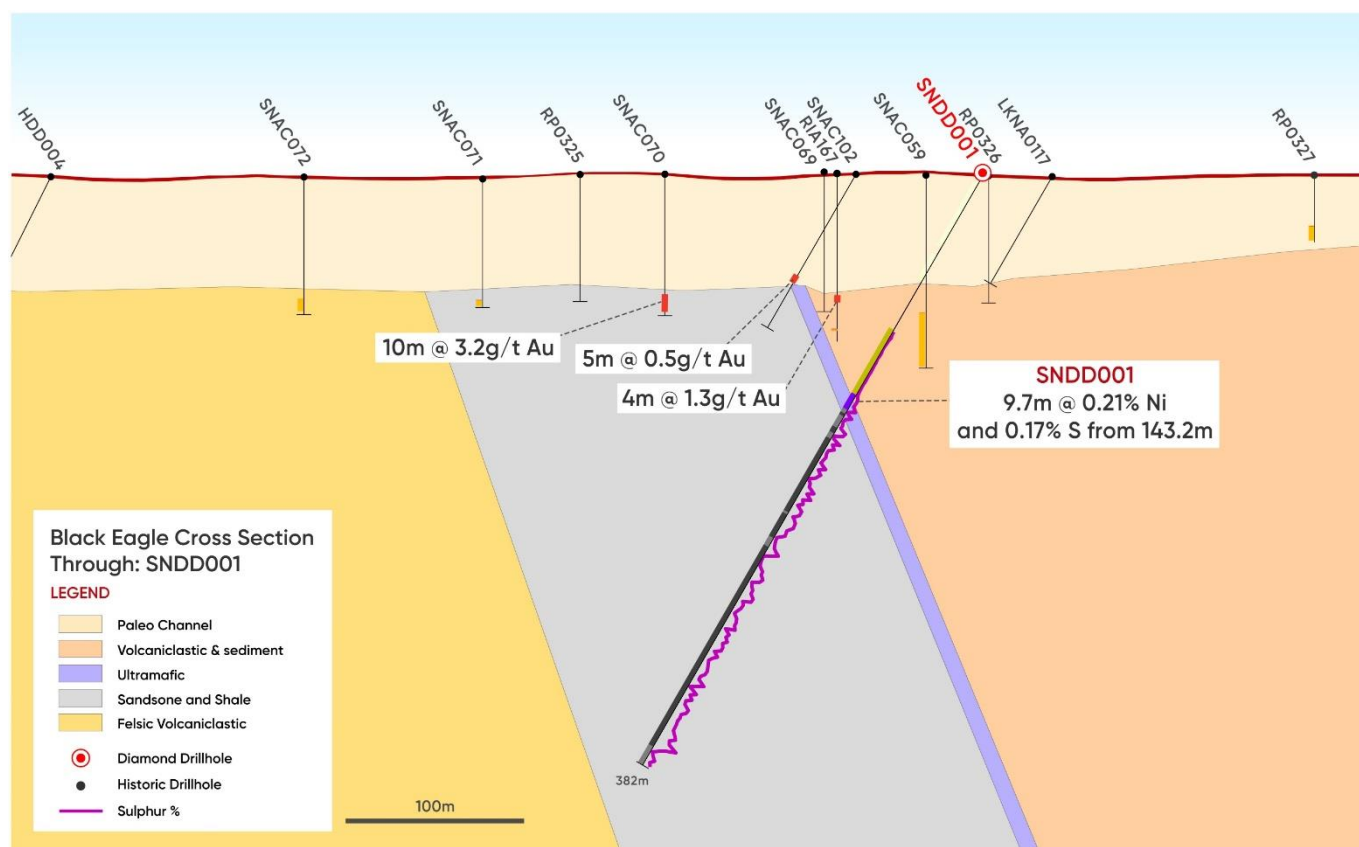
Figure 3. Schematic section of drilling (SNDD001) completed at Black Eagle
