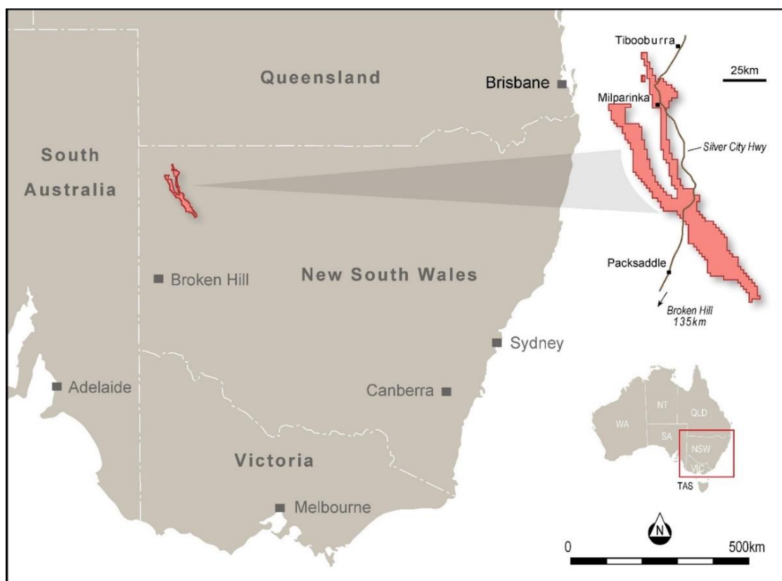
Figure 2: Location of the Tibooburra Gold Project.
