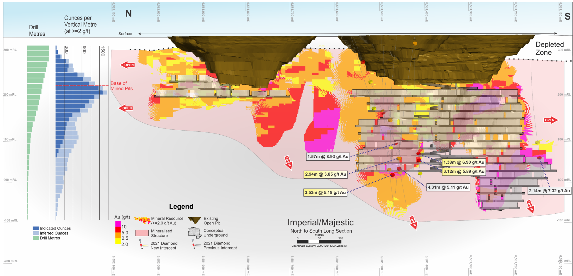
Figure 4: Long section showing Majestic and Imperial. Existing open pits (brown) and Resources >2.0 g/t Au are shown. Pink shadow indicates <2.0 g/t Au mineralised structure which remains of interest in a high-grade nuggety system. Planned initial underground development is overlain
