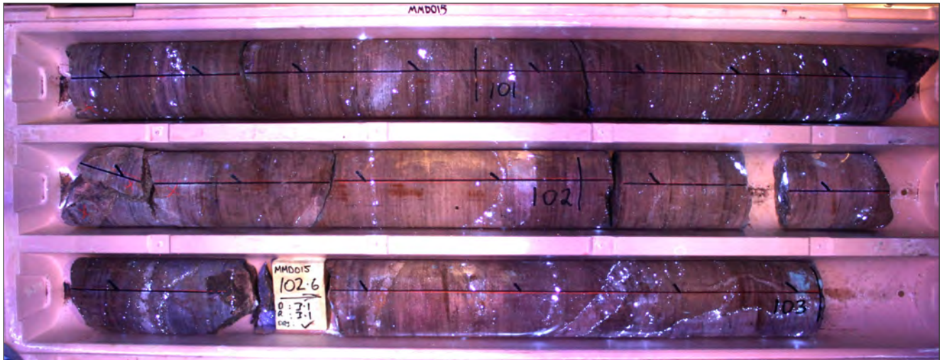
Figure 3. UV Photograph of typical mineralised core in MMD015 from 100.5m to 103.0m recovered from the current Mulgine Trench drilling program, showing coarse grained scheelite associated with quartz veining. The corresponding zone in the twin hole MMC319 assayed 4m at 0.11% WO 3 from 100m, within an overall mineralised envelope of 108m at 0.11% WO 3 , 70 ppm Mo from surface.
