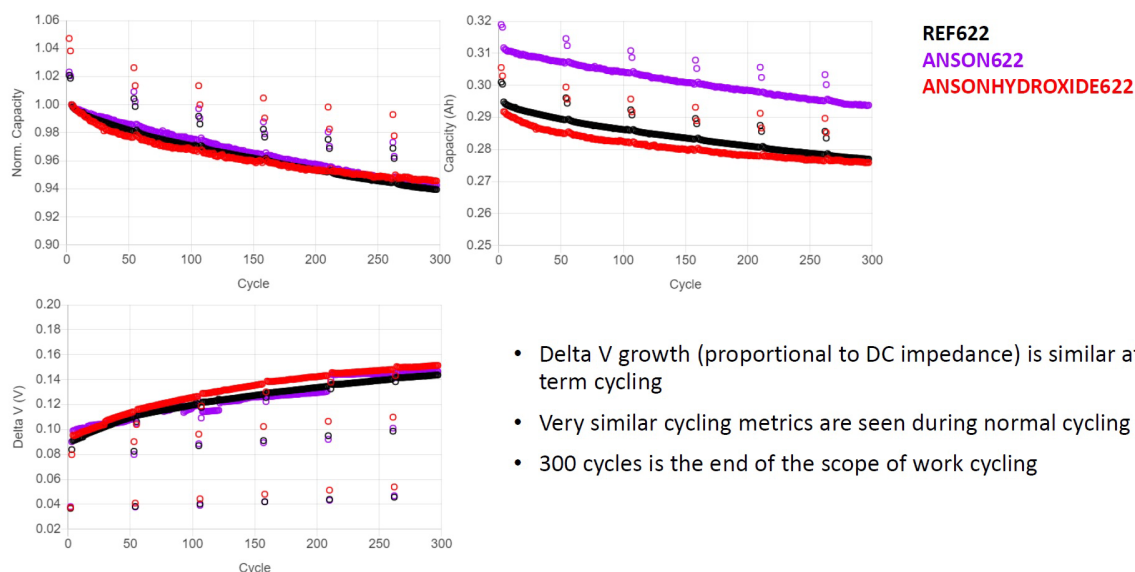
Figure 1: NOVONIX Long Term Cycling Test Work Results
