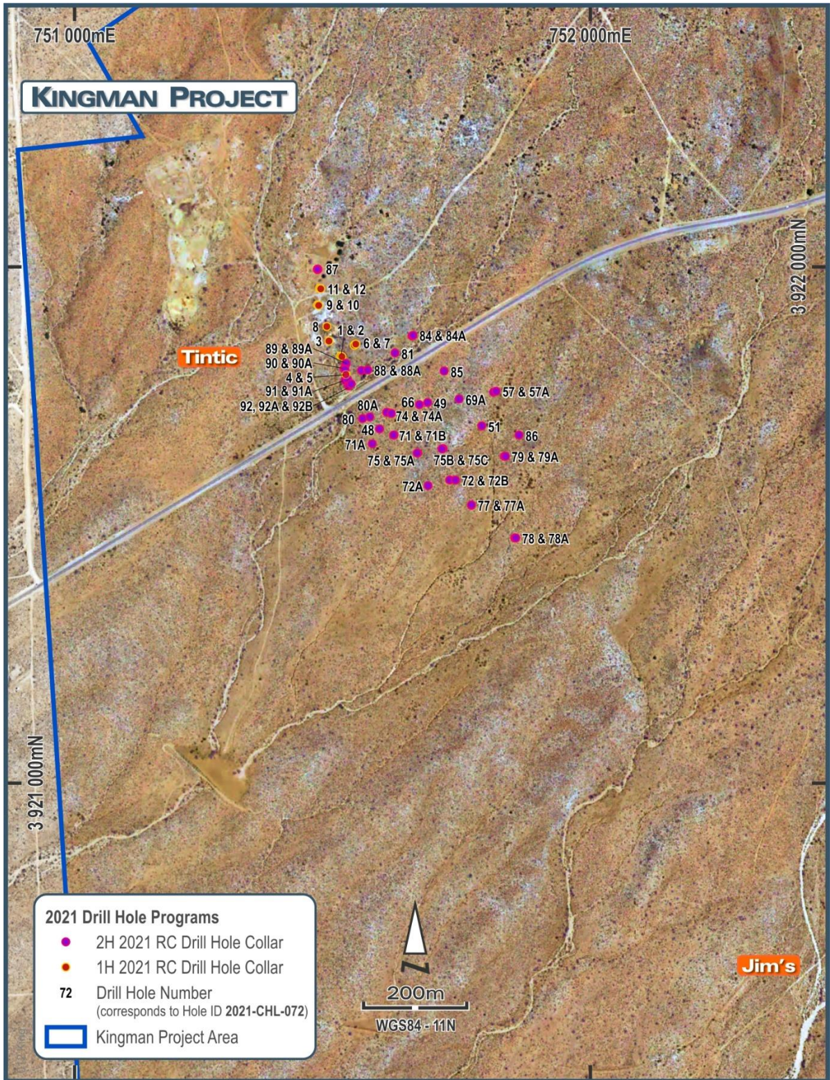
Figure 2 – RC Drill Collar locations at Tintic (September-October 2021) showing focus of current RC drill program
