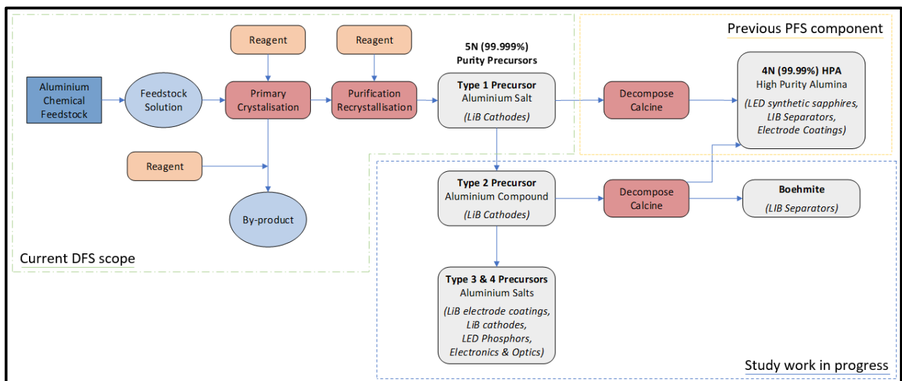
Overview Flowsheet
