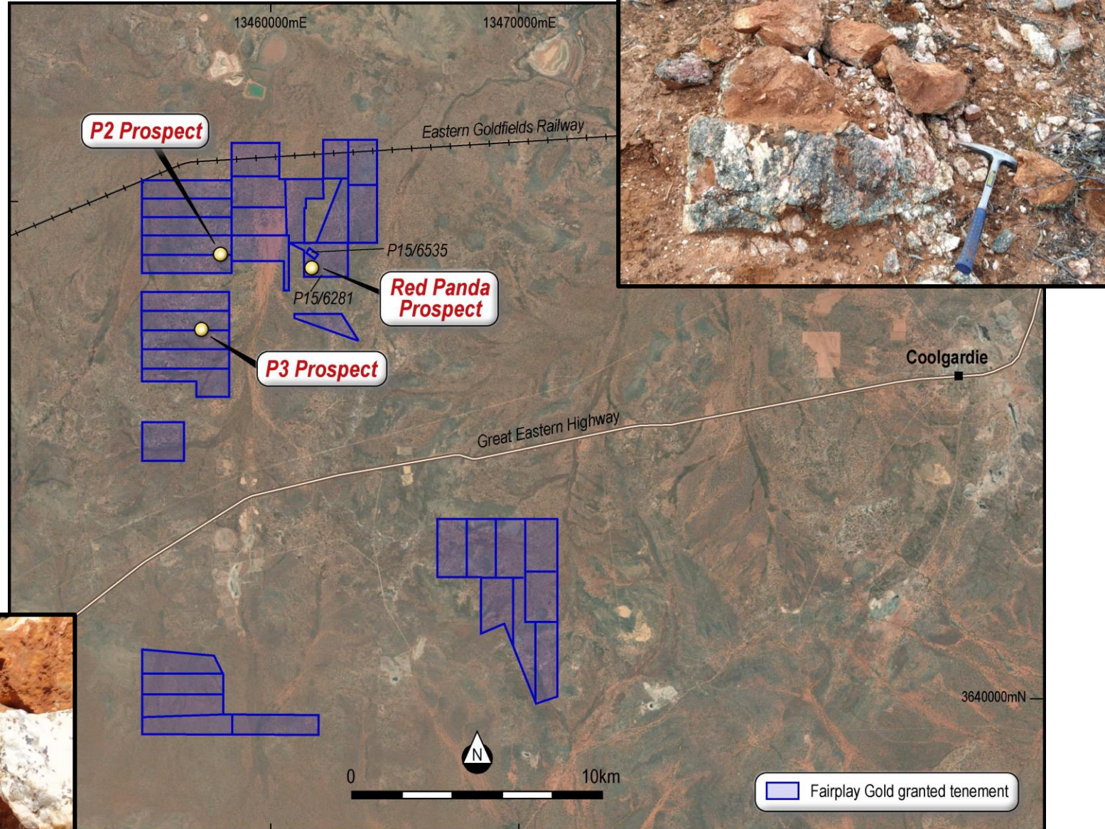
Red Panda Prospect perthitic quartz/feldspar/tantalite pegmatite
