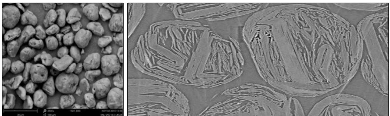
Figure 3: Spherical graphite (left) and cross sections through spherical graphite (right) Source: ProGraphite GmbH, Berlin 2017. The spheres are ~10-15 \mu\text{m} diameter
