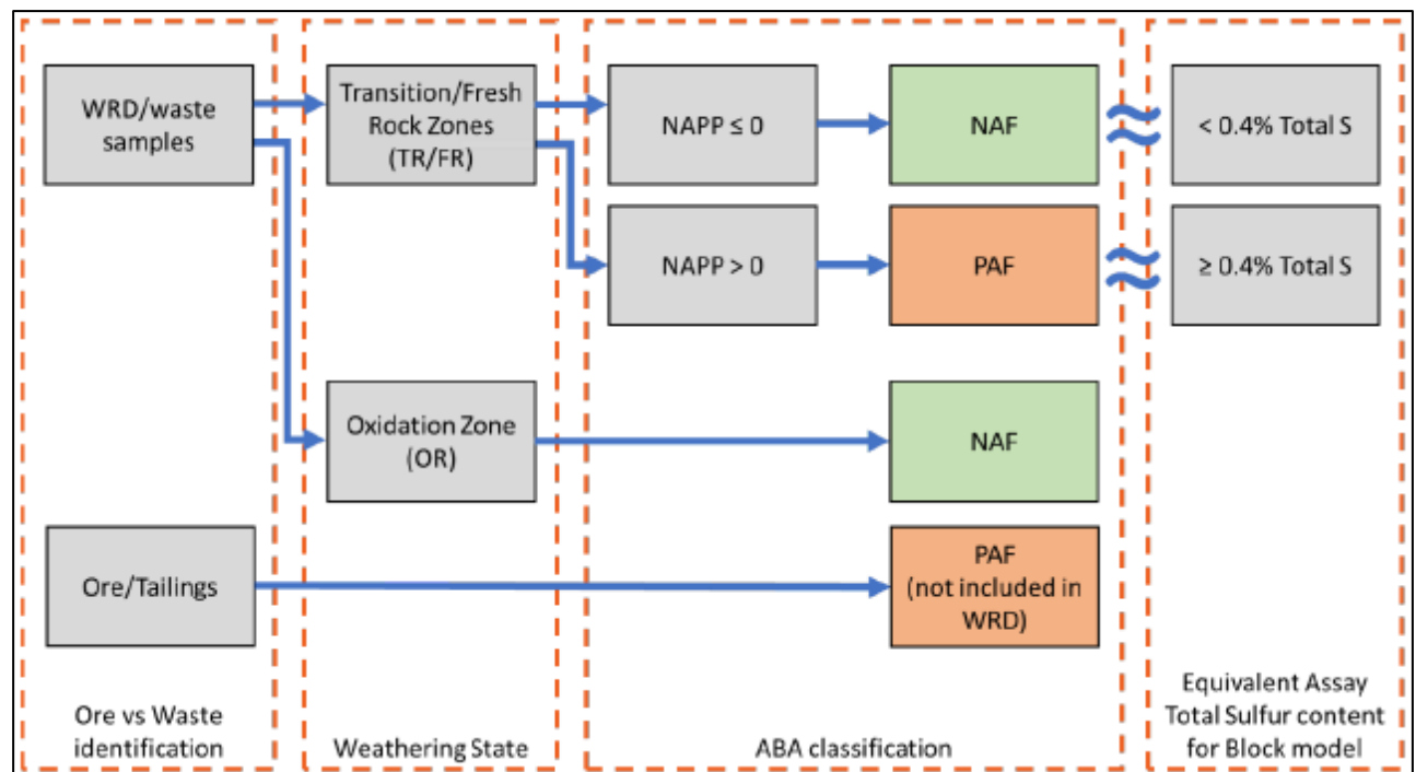
Figure 22: Waste rock AMD classification process
