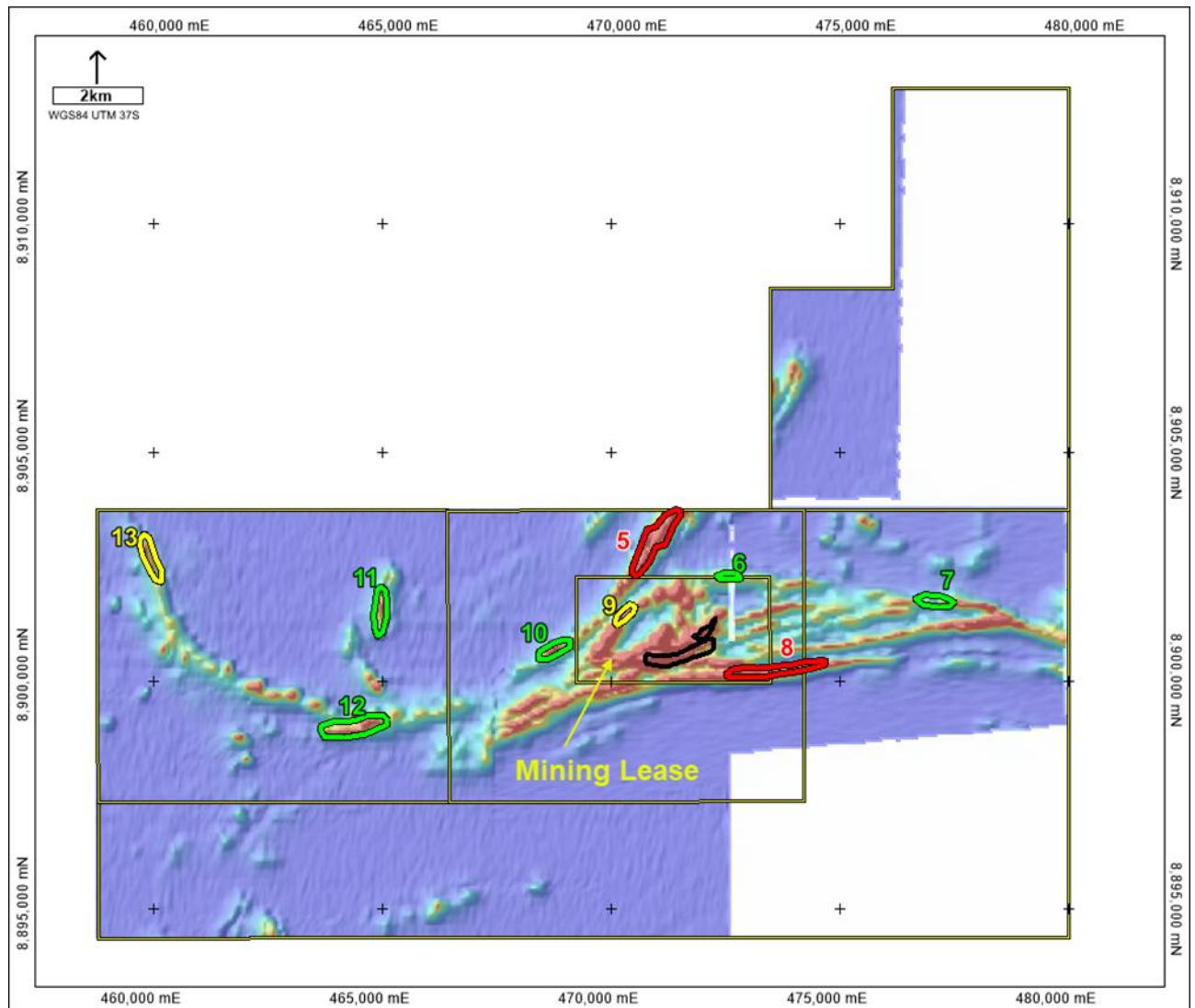
Figure 26: Map of the Chilalo tenements, showing conductive VTEM and FLEM targets The Chilalo Inferred MRE outline is shown as two black polygons, within the Mining Licence. The FLEM targets are ranked from high priority (red) to lower priority (green or yellow). Map sourced from Resource Potentials Pty Ltd (Sinnott, J., 2017 and 2019).
