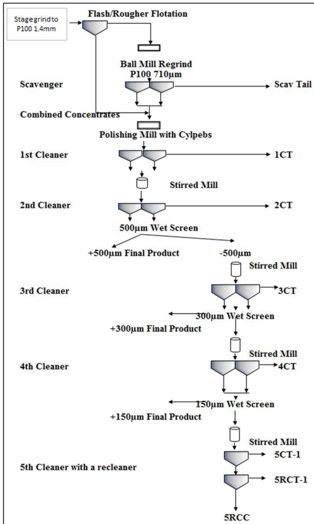
Figure 17: Final bench-scale optimised flowsheet
