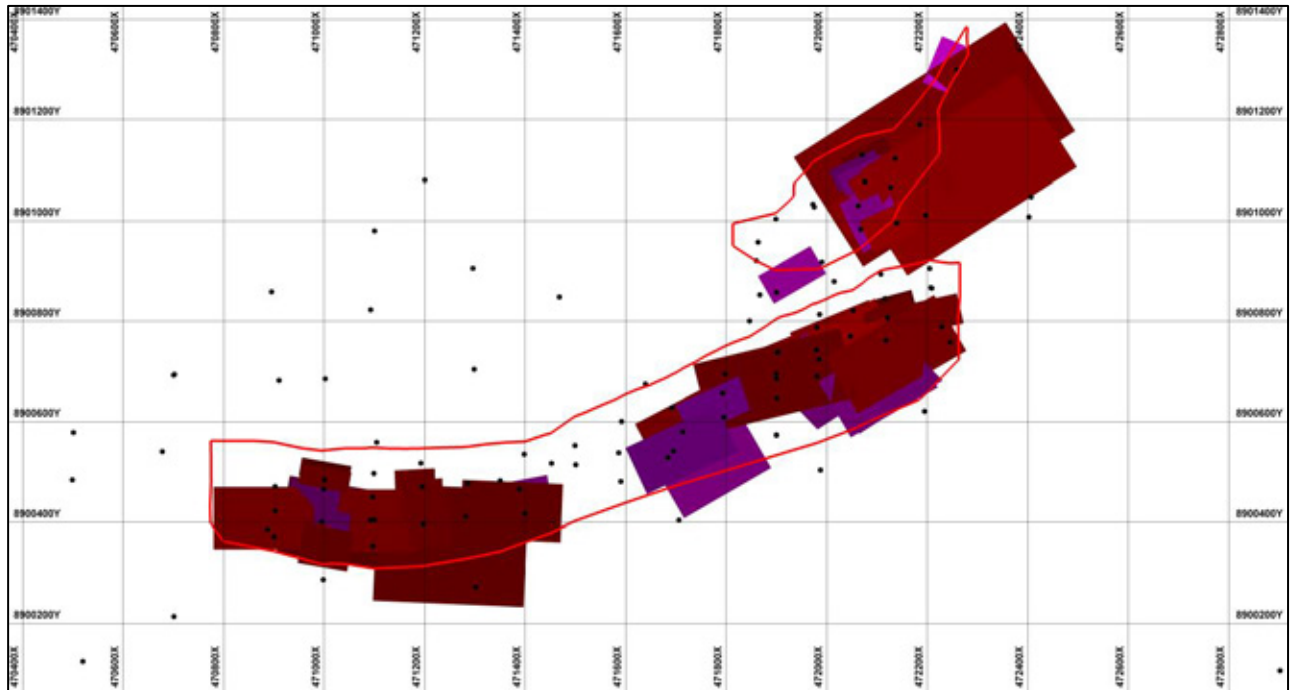
Figure 8: Map of very strong and strong DHEM conductor plates The plates are shown relative to the Chilalo Mineral Resource outline of August 2019. Map grid 200 m x 200 m.
