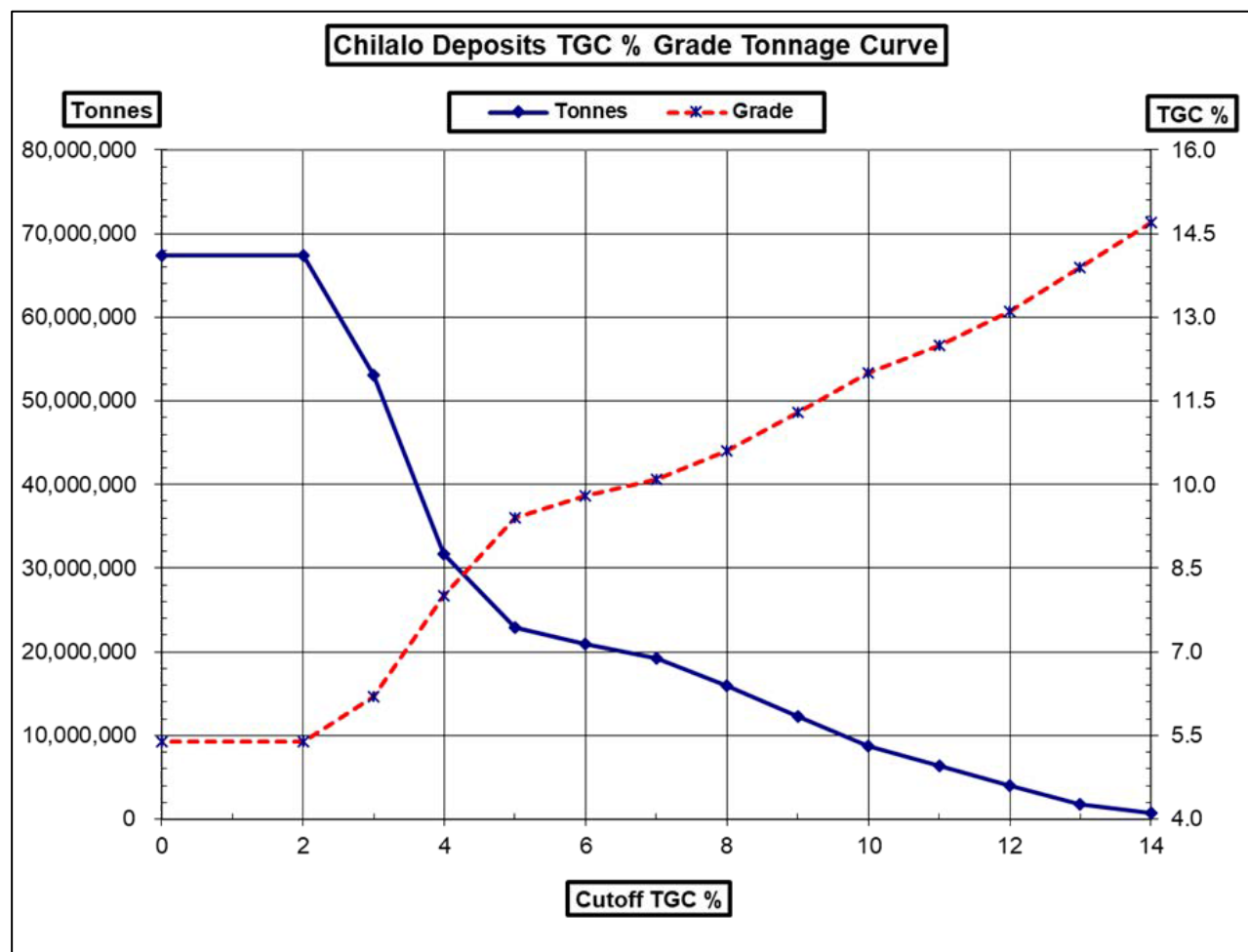
Figure 18: Grade-tonnage curves for the Chilalo deposit – all classified material
