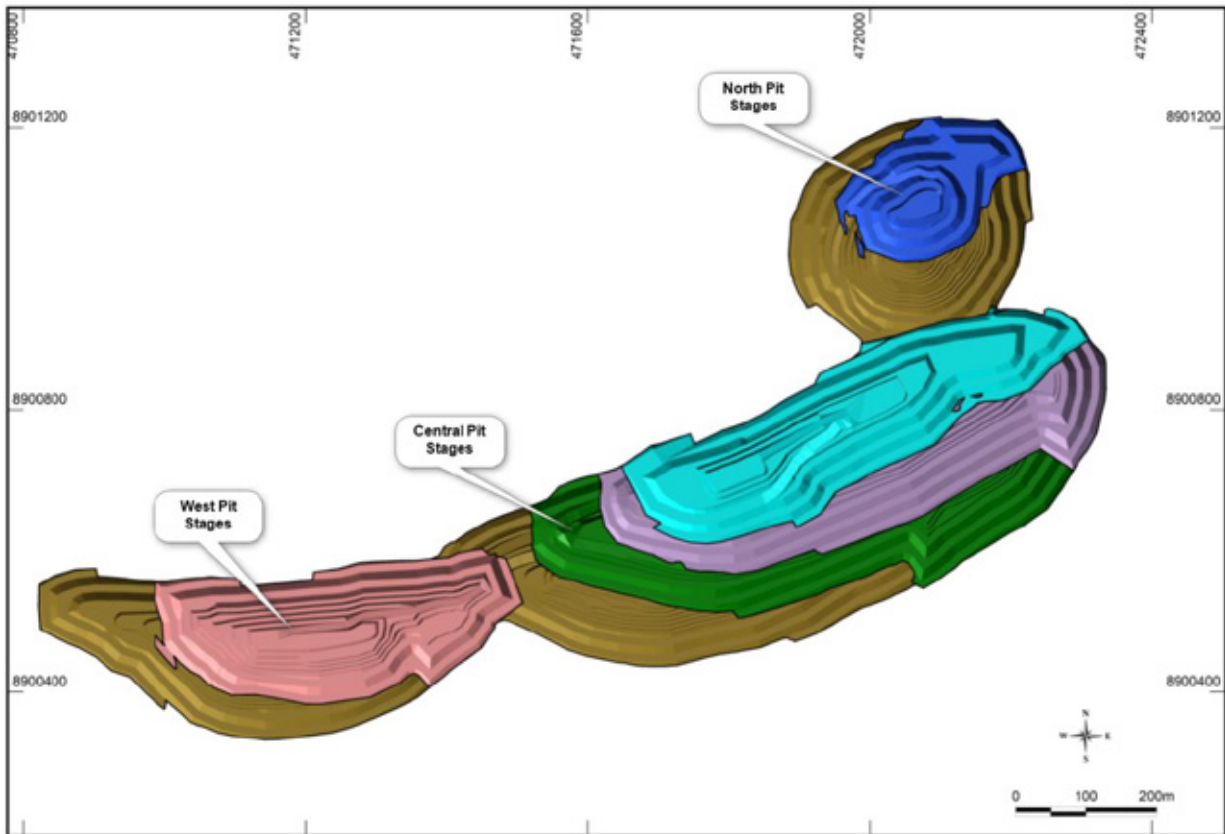
Figure 13: Chilalo Pit Design
