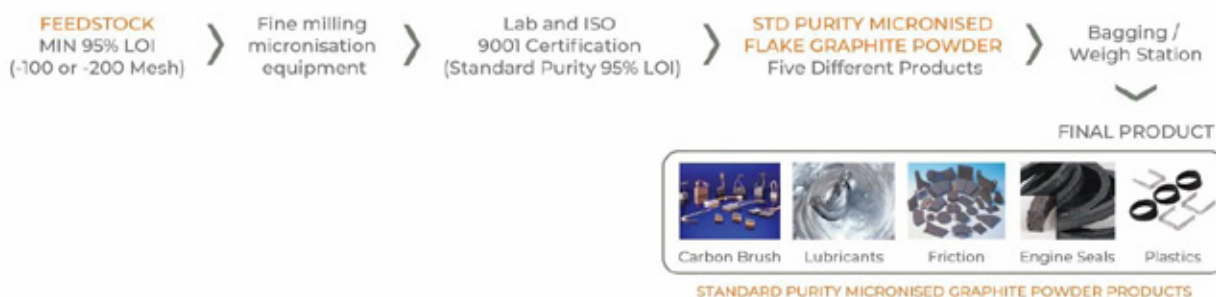
Figure 8: Process flow chart for micronised graphite
