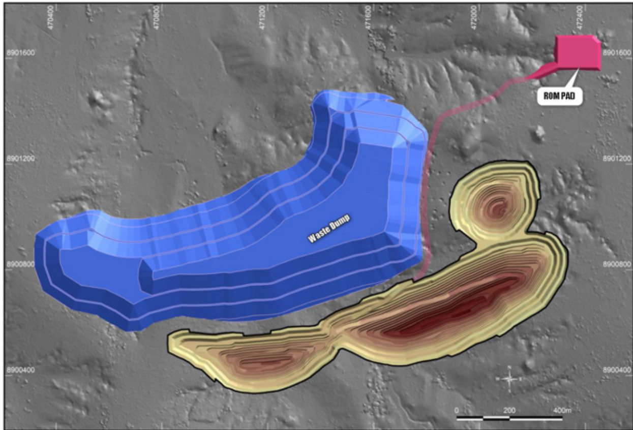
Figure 14: Final Pit, Waste Dump and ROM Pad Designs
