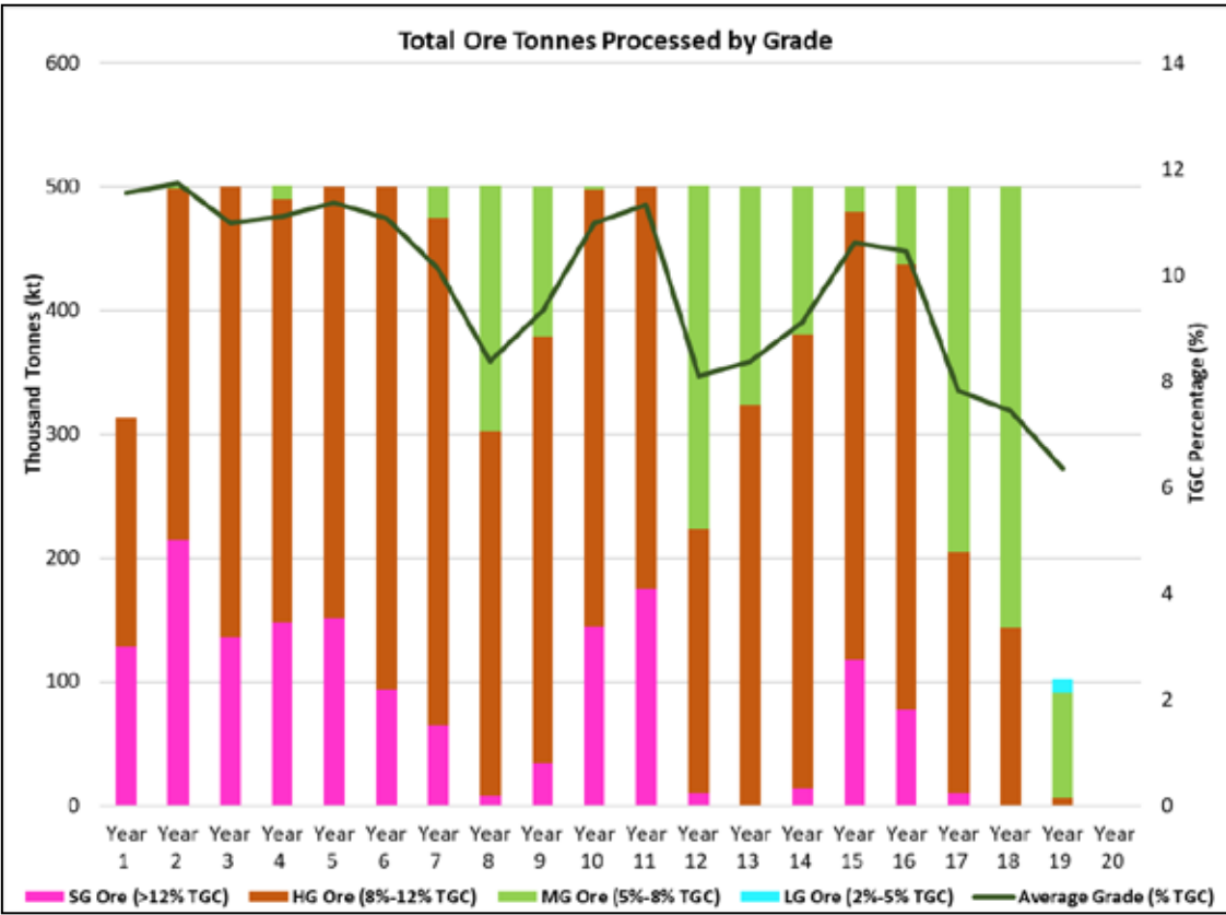
Figure 19: Total Ore Tonnes Processed by Grade
