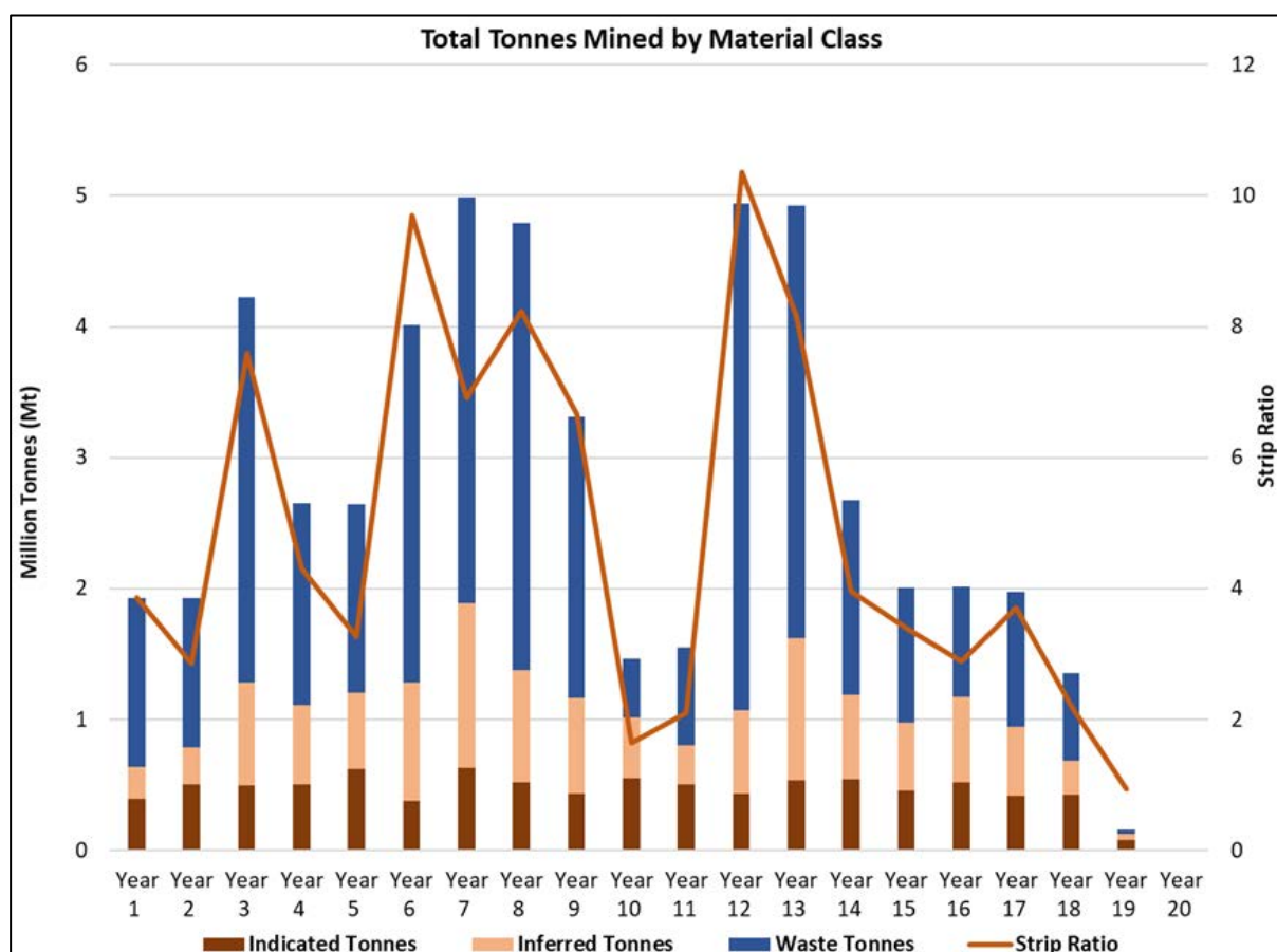
Figure 23: Total tonnes mined by material class
