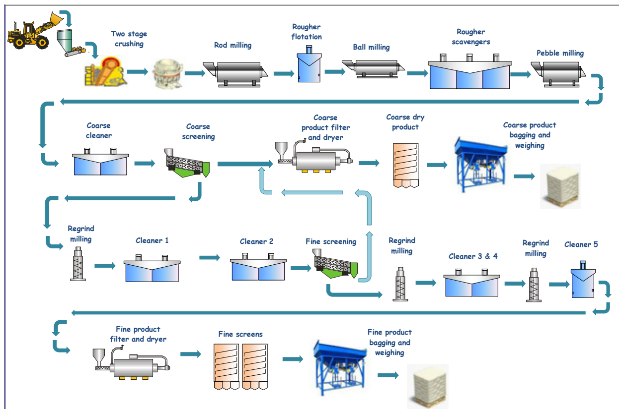
Figure 9. Simplified flow sheet
