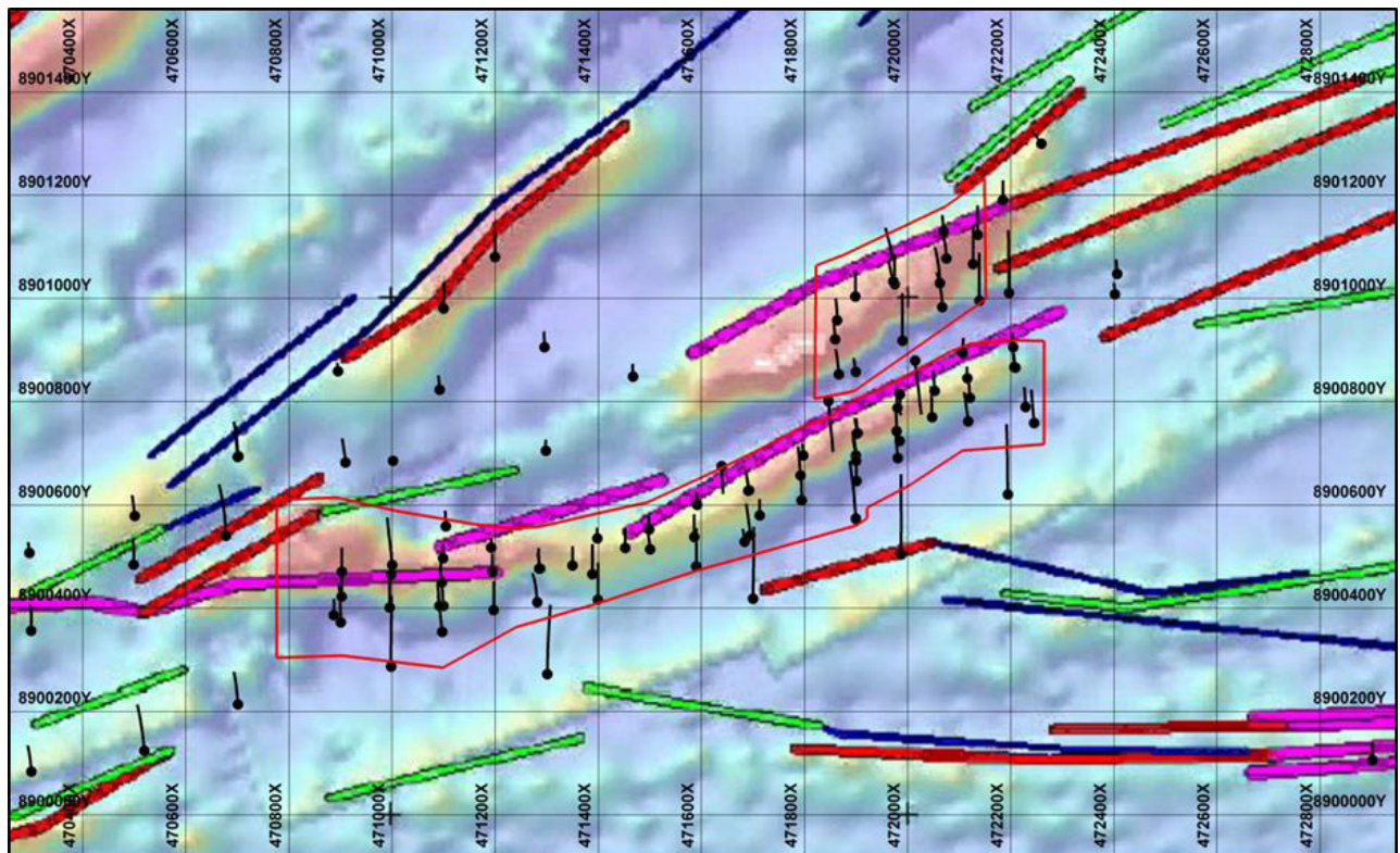
Figure 6: Detail of FLEM conductor plates projected to ground surface at the Chilalo deposit The 2017 Chilalo Mineral Resource outline is shown as a red polygon; drill collars and traces as black dots and lines. Map grid 200 m x 200 m. The underlying image shows the VTEM anomalies.
