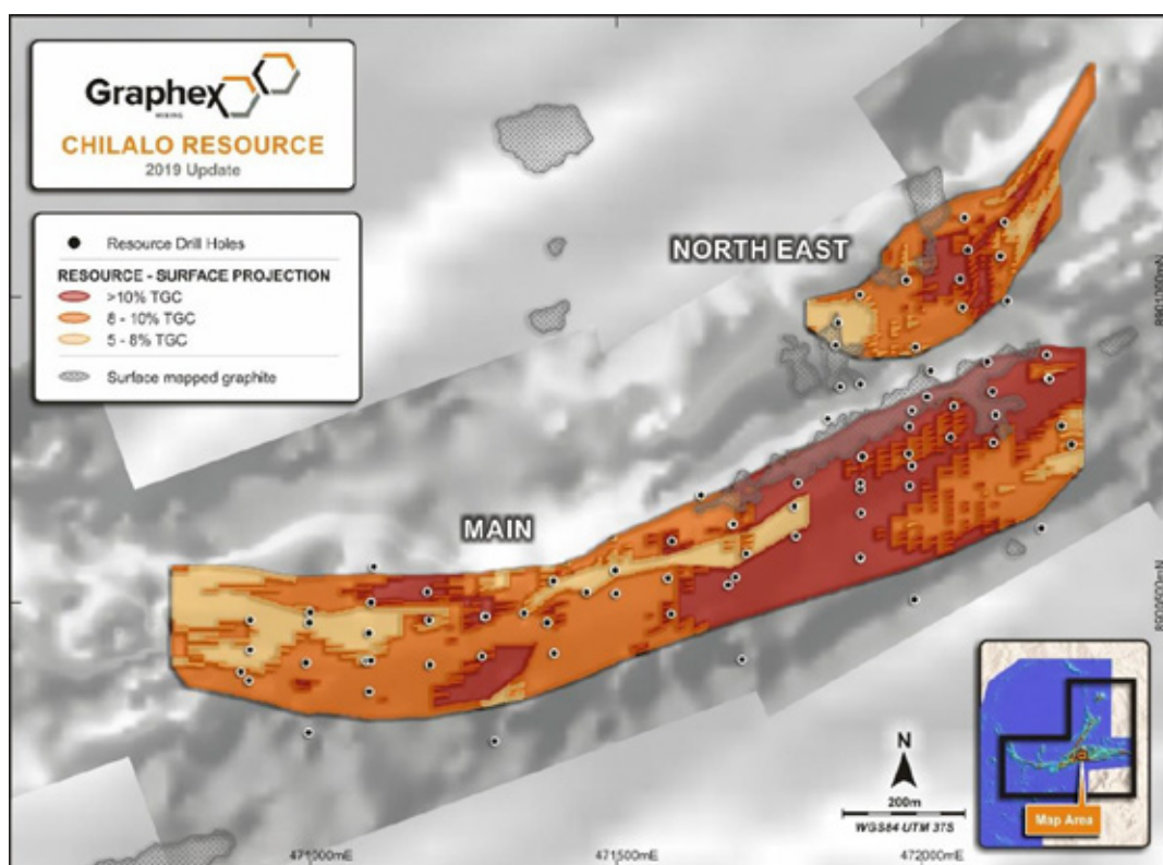
Figure 3. Image showing the grade of the high-grade resource
