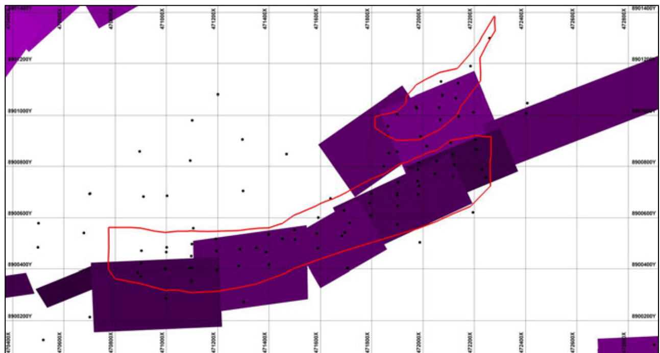
Figure 7: Map of very strong and strong conductance FLEM plates Chilalo Mineral Resource of August 2019 shown as red outline. Map grid 200 m x 200 m.
