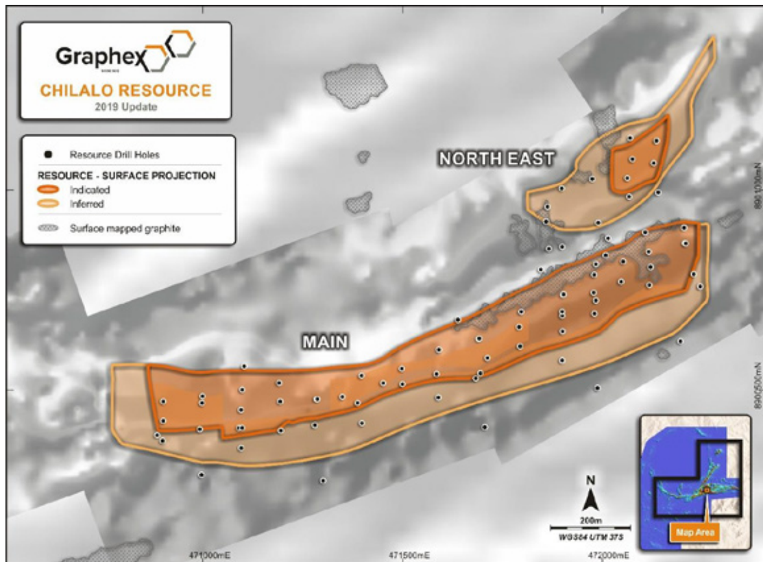
Figure 4. Classification of updated Chilalo Mineral Resource
