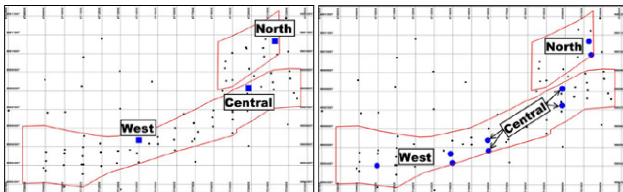
Figure 15: Location of drill collars for oxide (L) and fresh (R) global composites Red outline shows the approximate extent of modelled graphite mineralisation in 2017
