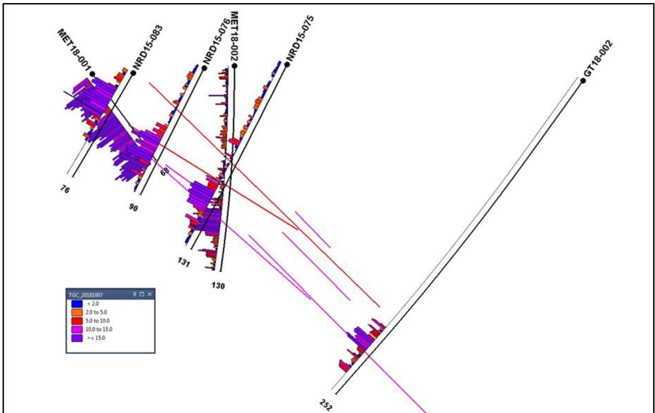
Figure 9: Cross section of the Central deposit showing modelled DHEM plates The very strong and strong plates extend through graphite intersected in drillholes. Section looking northeast, no vertical exaggeration. Purple = very strong; red = strong. Graphite values shown as bar charts along the borehole traces.
