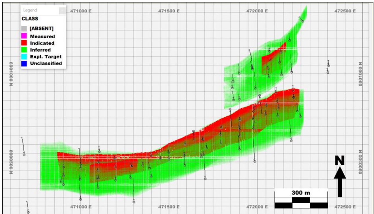
Figure 19: Plan view of classification (red = Indicated, green = Inferred) Main map grid 500 m x 500 m.
