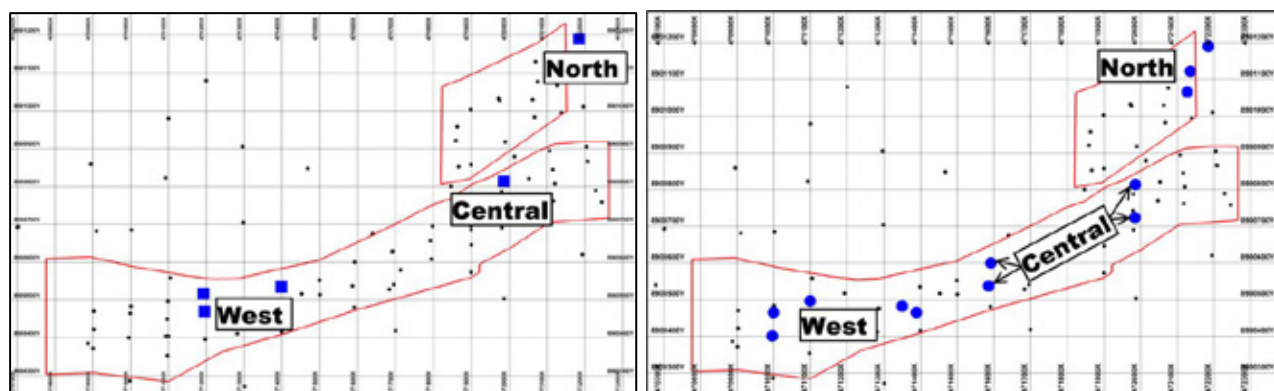
Figure 16: Location of drill collars for oxide(L) and fresh (R) variability composites
