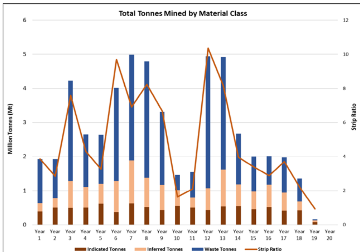
Figure 17: Total Tonnes Mined by Material Class
