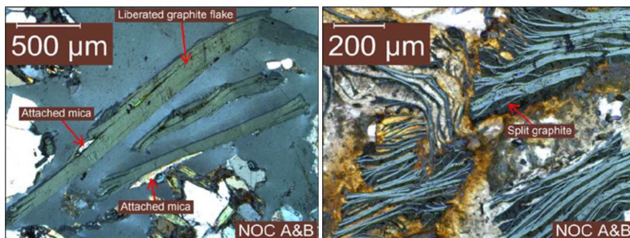
Figure 11: Photomicrographs of thin sections of North Oxide composite Left – large flake almost completely liberated. Right – split flakes in contact with clay minerals.
