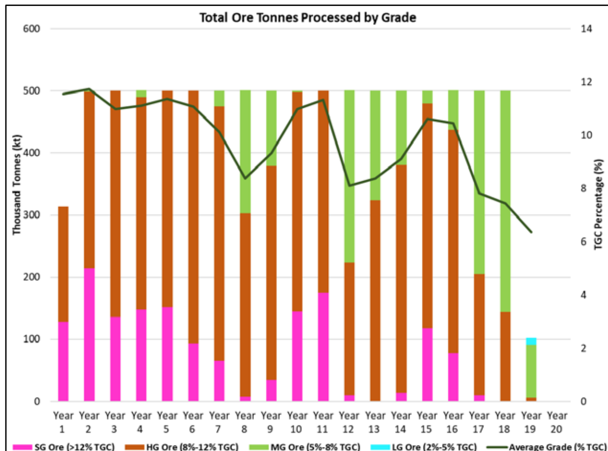
Figure 24: Total ore tonnes processed by grade
