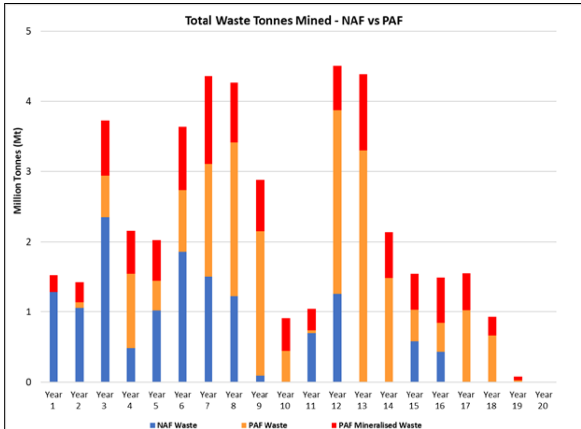
Figure 20: NAF and PAF Material Mined from Chilalo Pit
