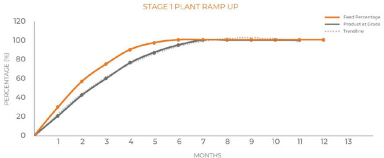
Figure 10. Chilalo processing plant commissioning assumptions
