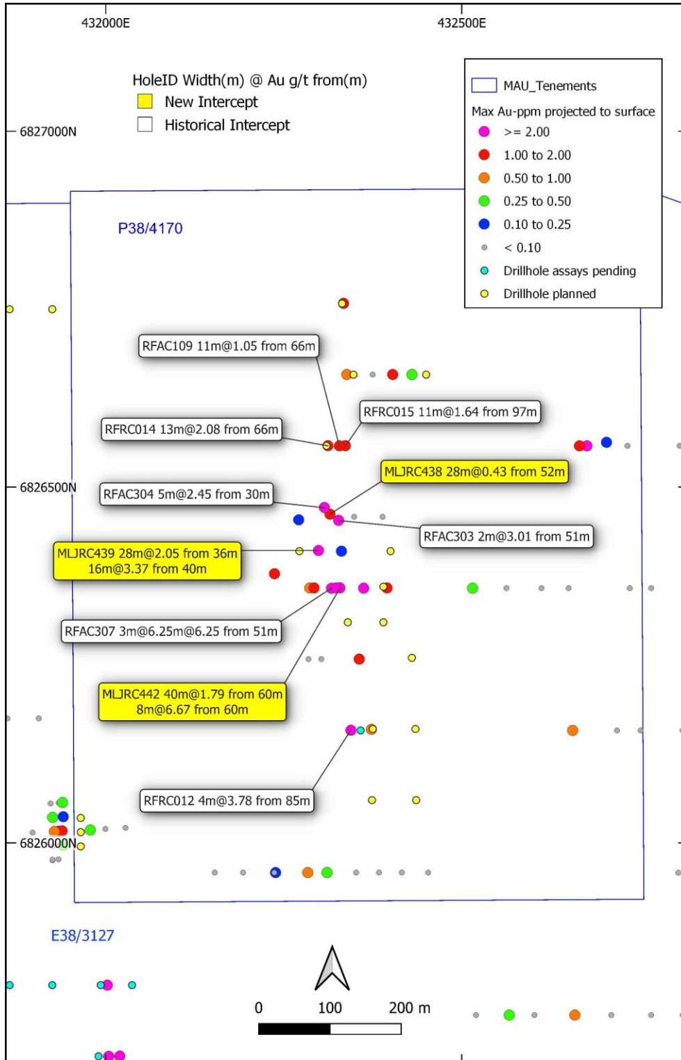
Figure 1. Lady Julie North 4 area highlighting significant thick intersections from the latest drill programme (yellow large rectangular label) and historical drilling (white labels) with maximum gold projected to surface and drillholes with assays pending (in blue) and planned drillholes (in yellow).
