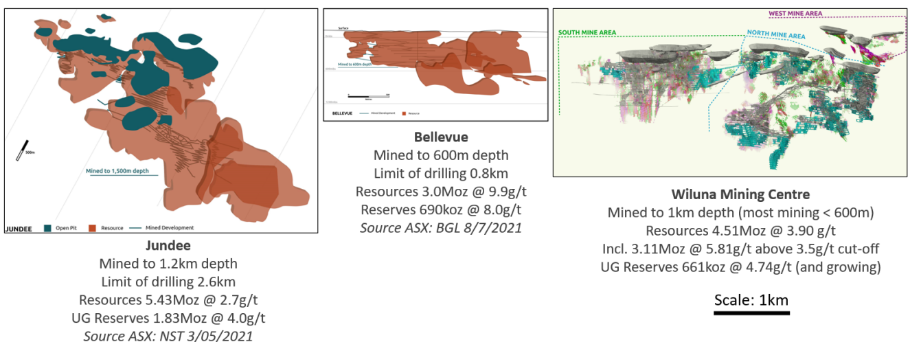
Figure 6: Large-scale gold projects with comparable resources and reserves.
