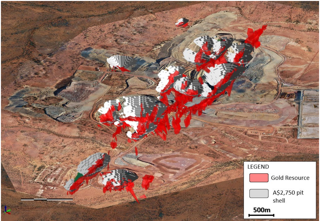
Figure 13: Matilda Mining Centre Mineral Resource, pit cut back optimisation shells and existing mine infrastructure with aerial photo; oblique view looking northwest.
