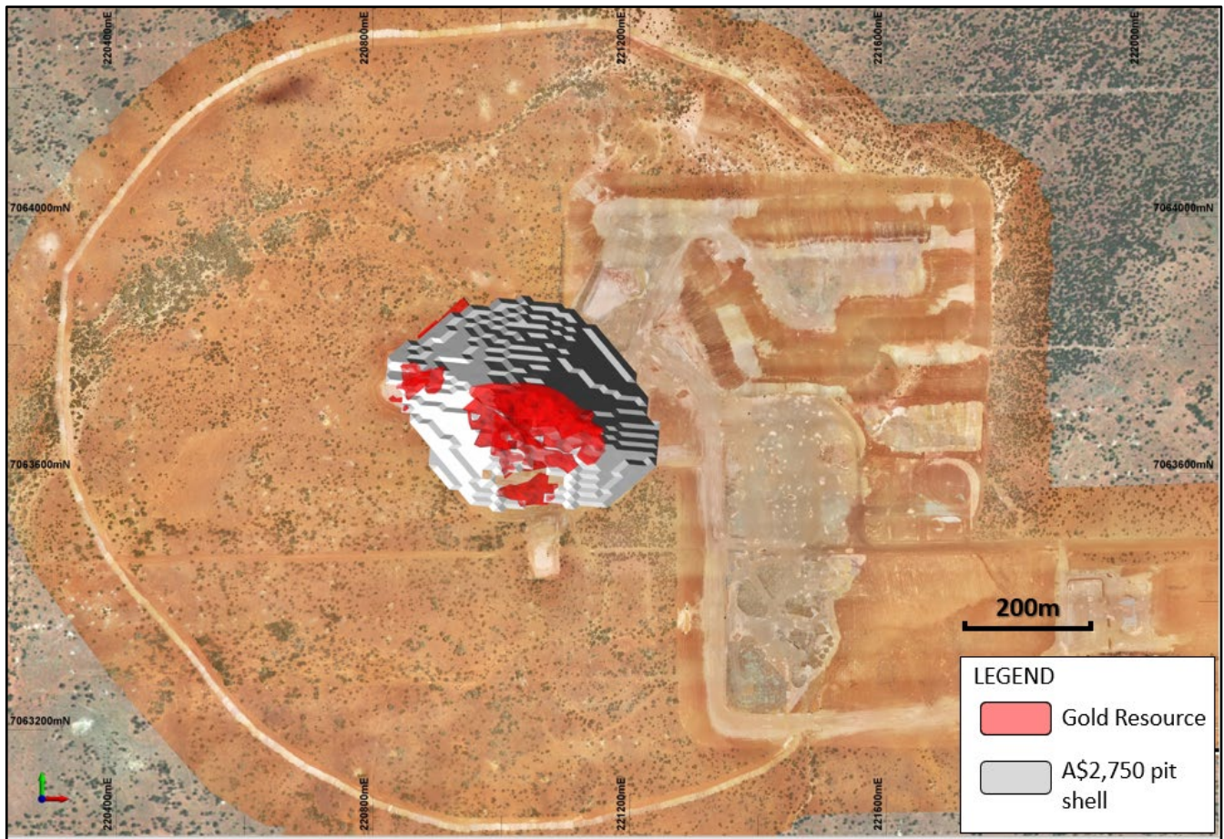
Figure 14: Galaxy Mineral Resource, pit cut back optimisation shell and existing mine infrastructure.
