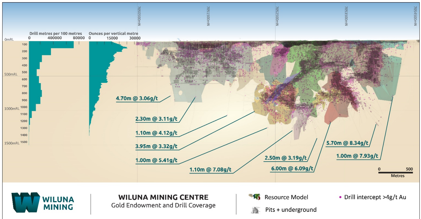
Figure 2. Wiluna Mining Centre drilling intensity chart and ounces per vertical metre; long section view looking west.
