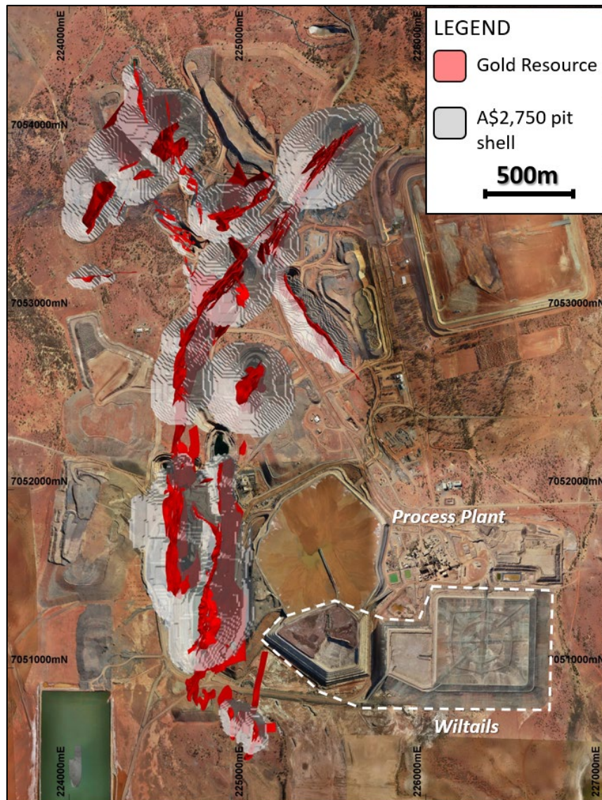
Figure 8: Wiluna Mining Centre mineralisation interpretations, A$2,750 pit optimisation shells and site layout, plan view.
