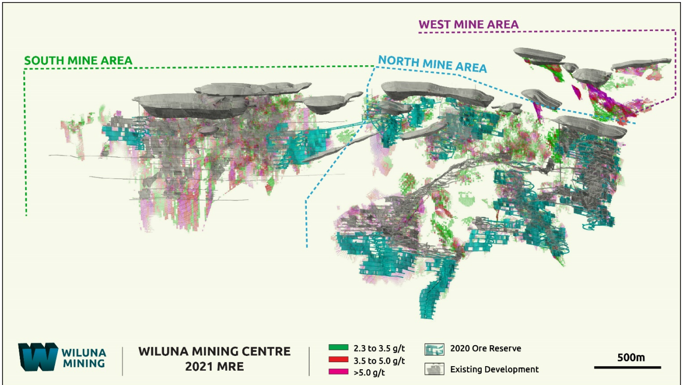
Figure 4: Mineral Resource coloured by grade, showing significant high-grade zones adjacent to the 2020 Ore Reserves; potential for additional Ore Reserves to be defined based on the updated MRE.
