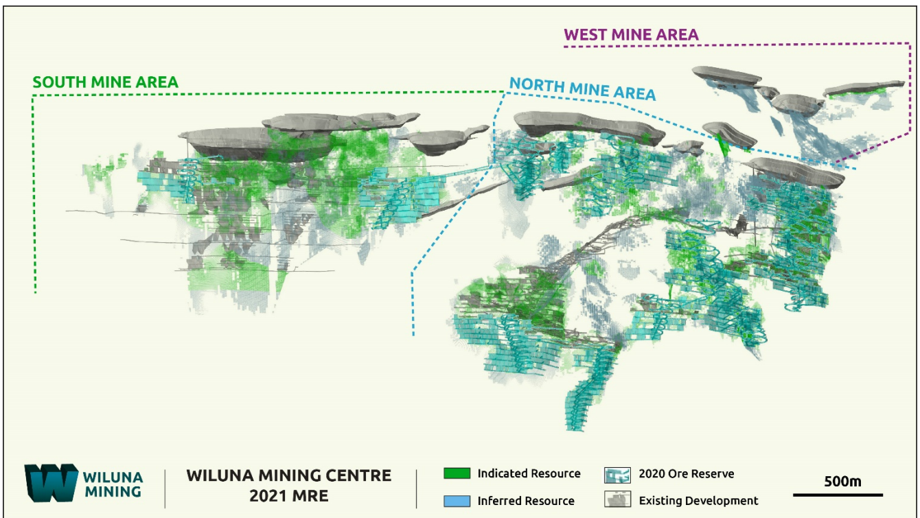
Figure 5: Mineral Resource coloured by category, showing significant Indicated zones adjacent to the 2020 Ore Reserves; potential for additional Ore Reserves to be defined based on the updated MRE.
