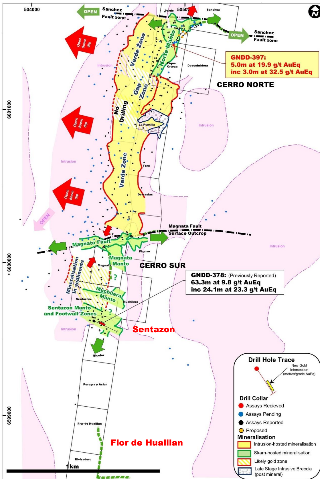
Figure 2 - Plan View Hualilan Project showing GNDD-397 Location
