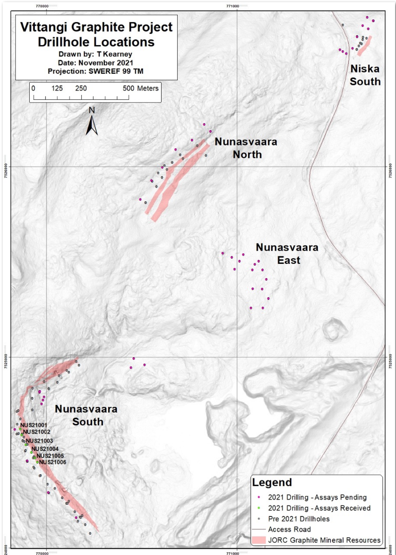
Figure 3 Vittangi Graphite Project drillhole and deposit locations.
