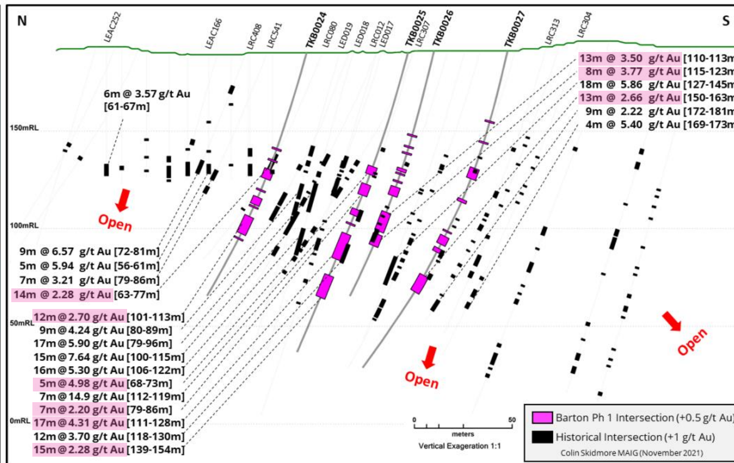
Tunkillia Central Area 223 Long Section with Significant Intersections 2
