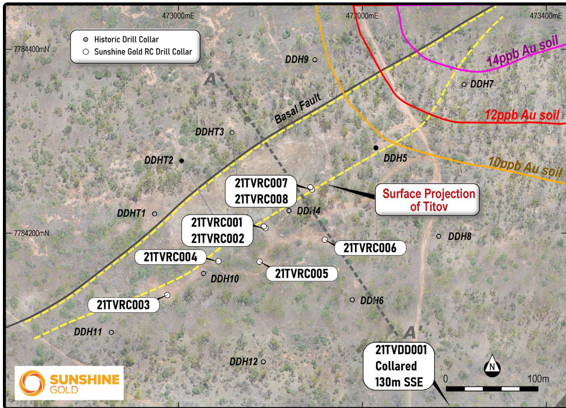
Figure 3. Collar positions and interpreted lode at surface, Titov.
