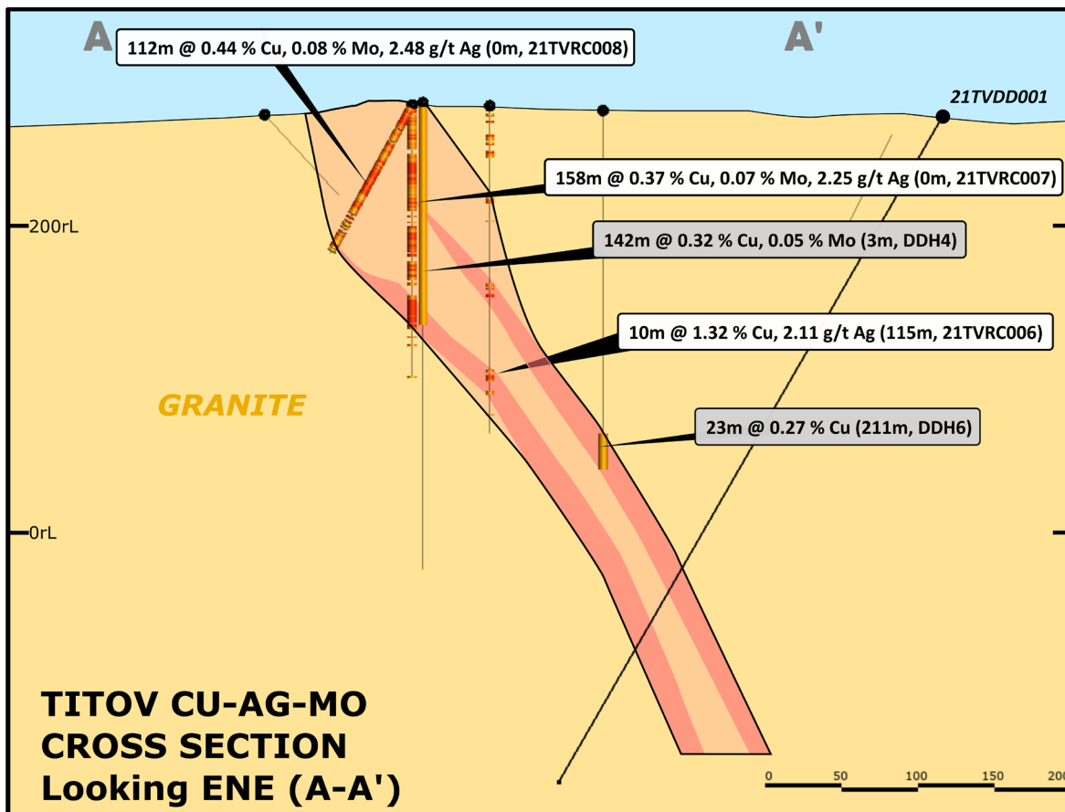
Figure 4. Cross Section displaying eastern RC holes and current diamond hole, Titov.
