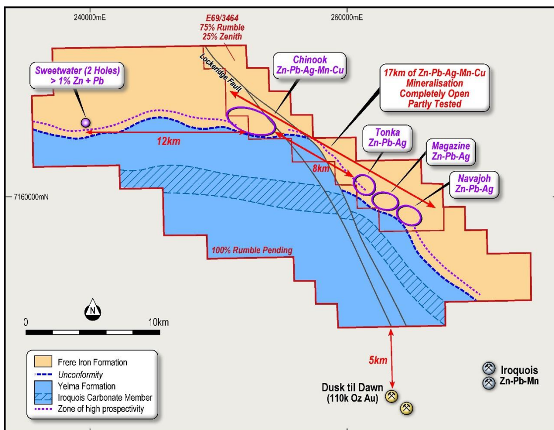
Image 1. Earacheedy Project – Geology and Location of Prospects
