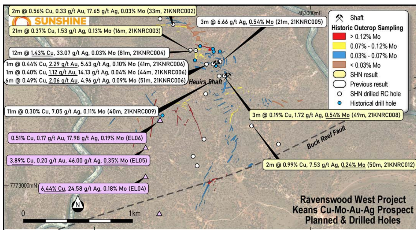
Figure 2. Location of recent significant RC intersections (yellow & white) and rock chip samples (purple).
