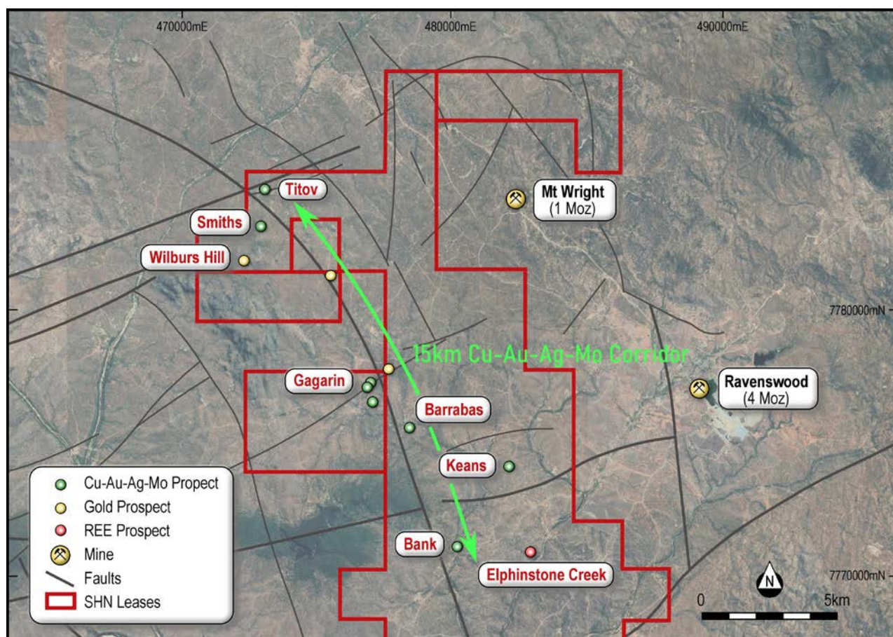
Figure 1. Map of the >15km long Cu-Au-Ag-Mo corridor at Ravenswood West.
