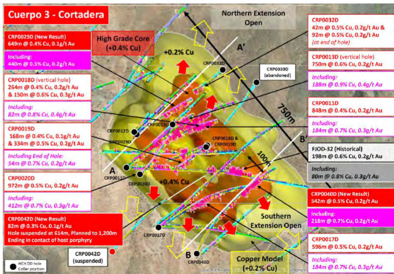
Figure 21 Plan view of Cuerpo 3 - the Main porphyry of the four porphyry centres discovered to date at Cortadera. The plan displays the location and basic geology of the mineralised tonalitic host porphyry in relation to the location of significant results returned by Hot Chili during the first quarter of 2020. Note the growing extent of the modelled higher grade copper zone (red wireframe - +0.4% Cu) and the location of open boundaries for growth of the bulk copper envelope at Cortadera (yellow wireframe - +0.2% Cu).
