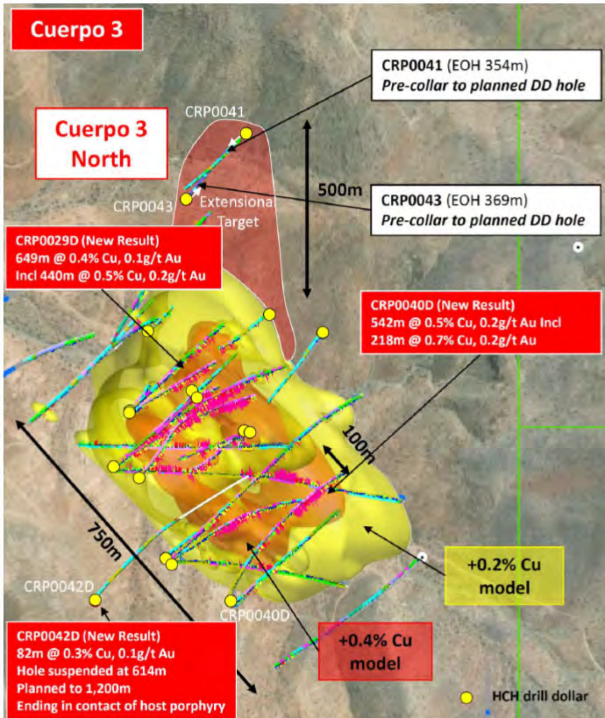
Figure 20 Plan view of Cuerpo 3 - the Main porphyry of the four porphyry centres discovered to date at Cortadera. The plan displays the location of significant results returned by Hot Chili during the first quarter of 2020. Note the growing extent of the modelled higher grade copper zone (red wireframe - +0.4% Cu) and the location of open boundaries for growth of the bulk copper envelope at Cortadera (yellow wireframe - +0.2% Cu)
