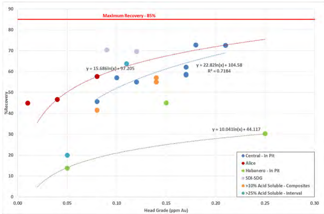
Figure 14 Gold head grade vs Recovery
