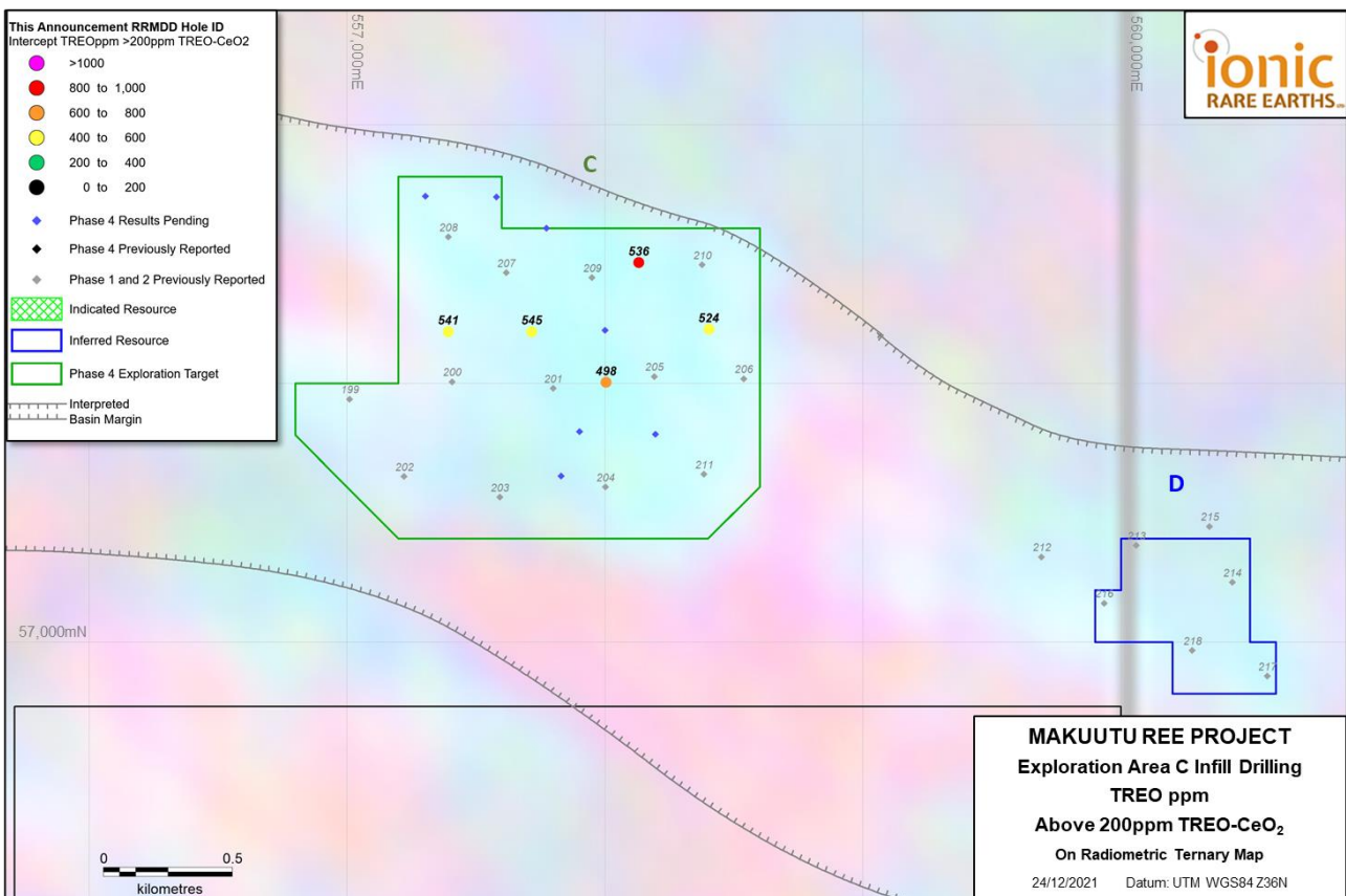
Figure 4: Exploration Area C drill plan with Tranche 4 infill drill holes showing hole locations by drill intercept TREO grade and RRMD drill hole ID. Pending holes in blue and Phase 1 and 2 holes in grey.
