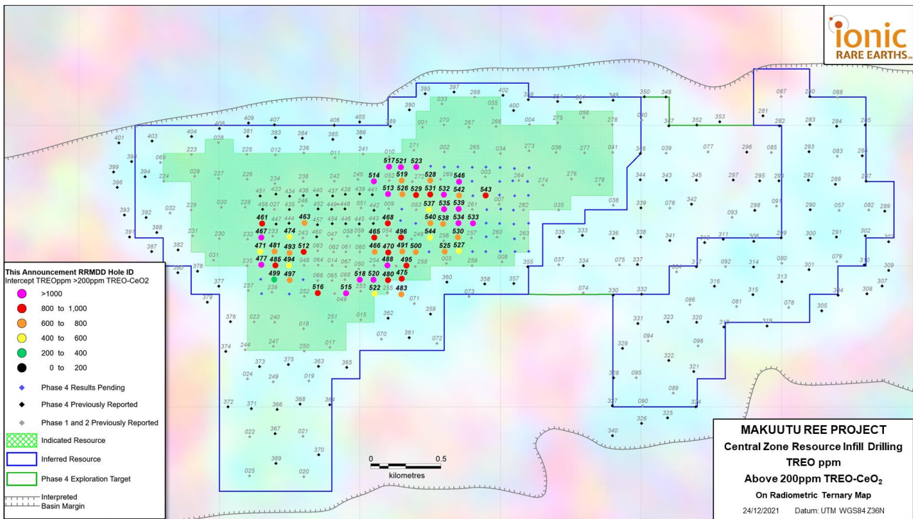
Figure 2: Makuutu Central Zone drill plan with Tranche 4 infill drill holes showing hole locations by drill intercept TREO grade and RRMD drill hole ID.
