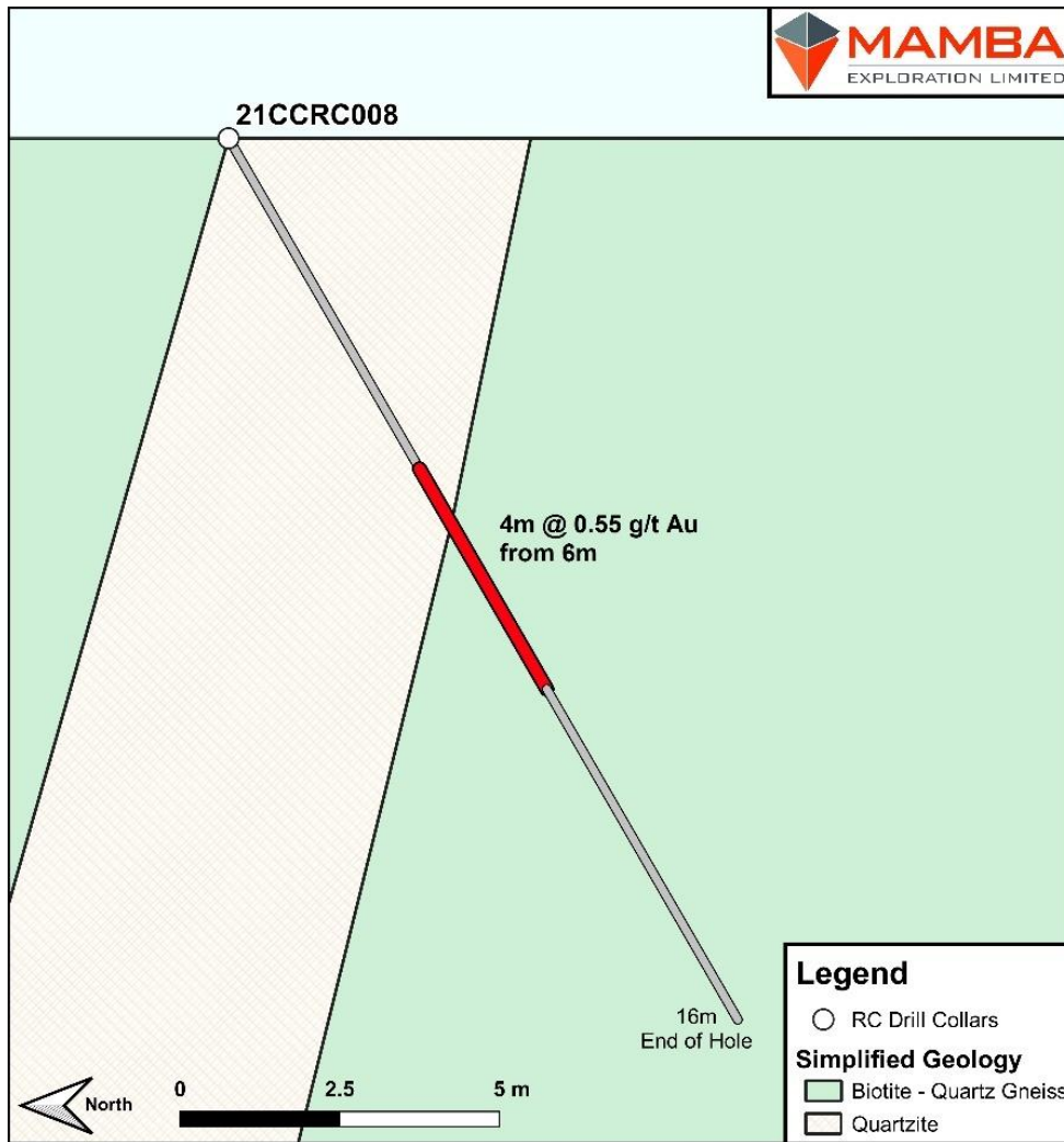
Figure 6: Southern Prospect RC Drilling Schematic Cross Section 691900mE
