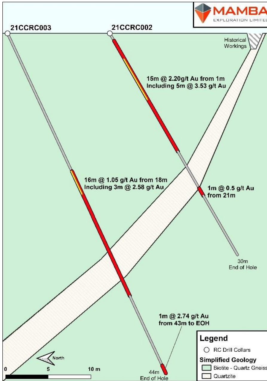
Figure 3: Southern Prospect RC Drilling Schematic Cross Section 691805mE
