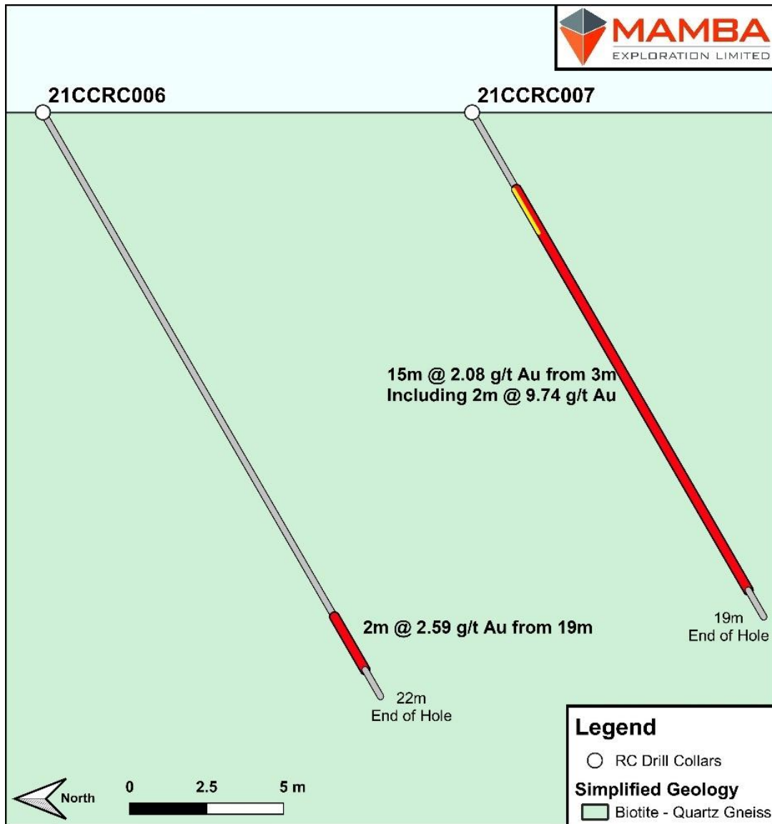
Figure 5: Southern Prospect RC Drilling Schematic Cross Section 691860mE
