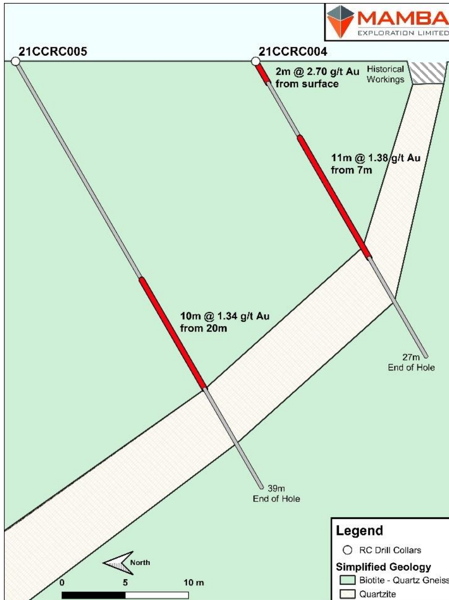
Figure 4: Southern Prospect RC Drilling Schematic Cross Section 691825mE
