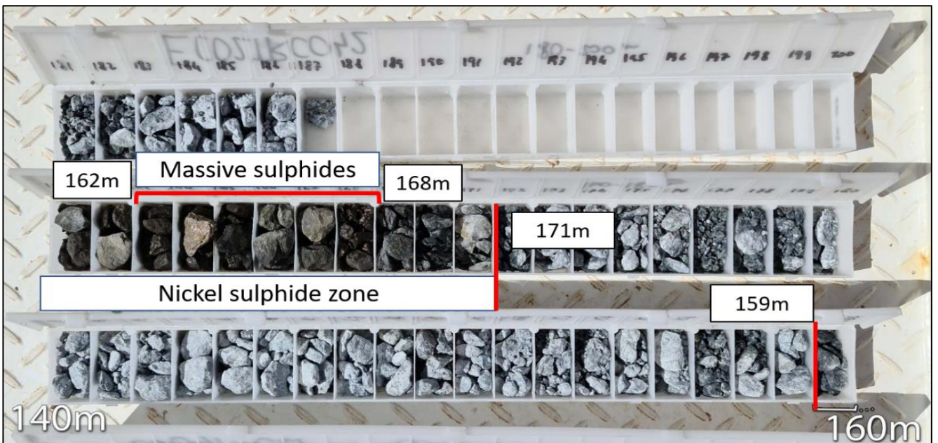
Figure 4 : RC Chip trays for ECO21RC_042 illustrating visual nickel sulphide zones of mineralisation: 10m @ 6.82% Ni incl: 6m @ 9.1% Ni
