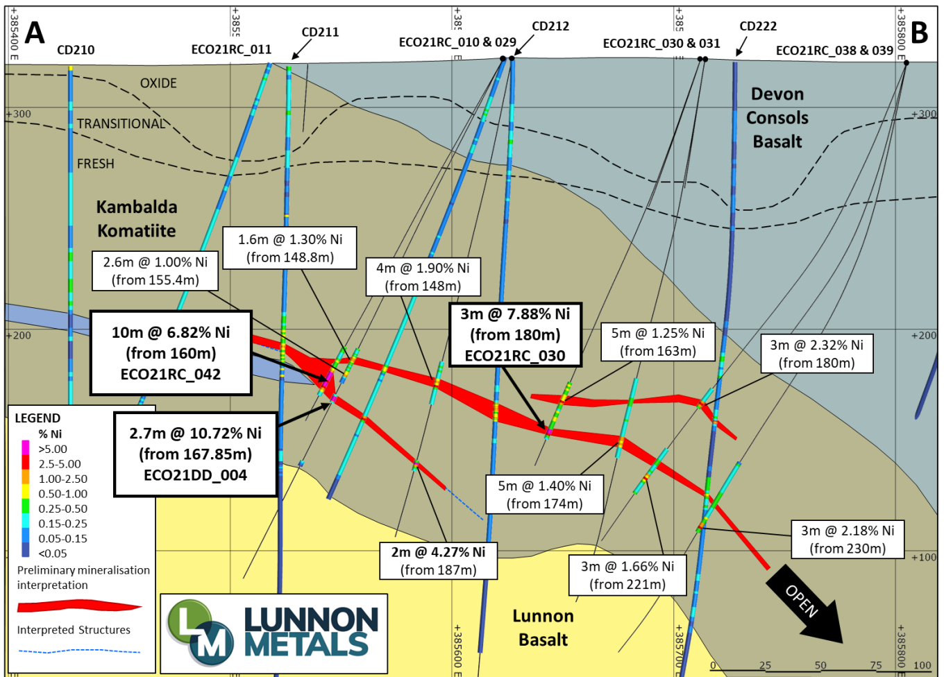
Figure 2: Cross section A-B (6,531,160mN) through Baker RC infill drilling, including previous drilling (looking north: Grid:MGA94_51) 2
