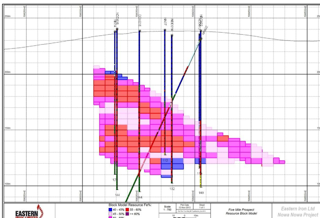
Figure 4 – Cross Section of the Five Mile Mineralisation Showing Estimated Blocks and Drill Hole Assays by Iron Grade
