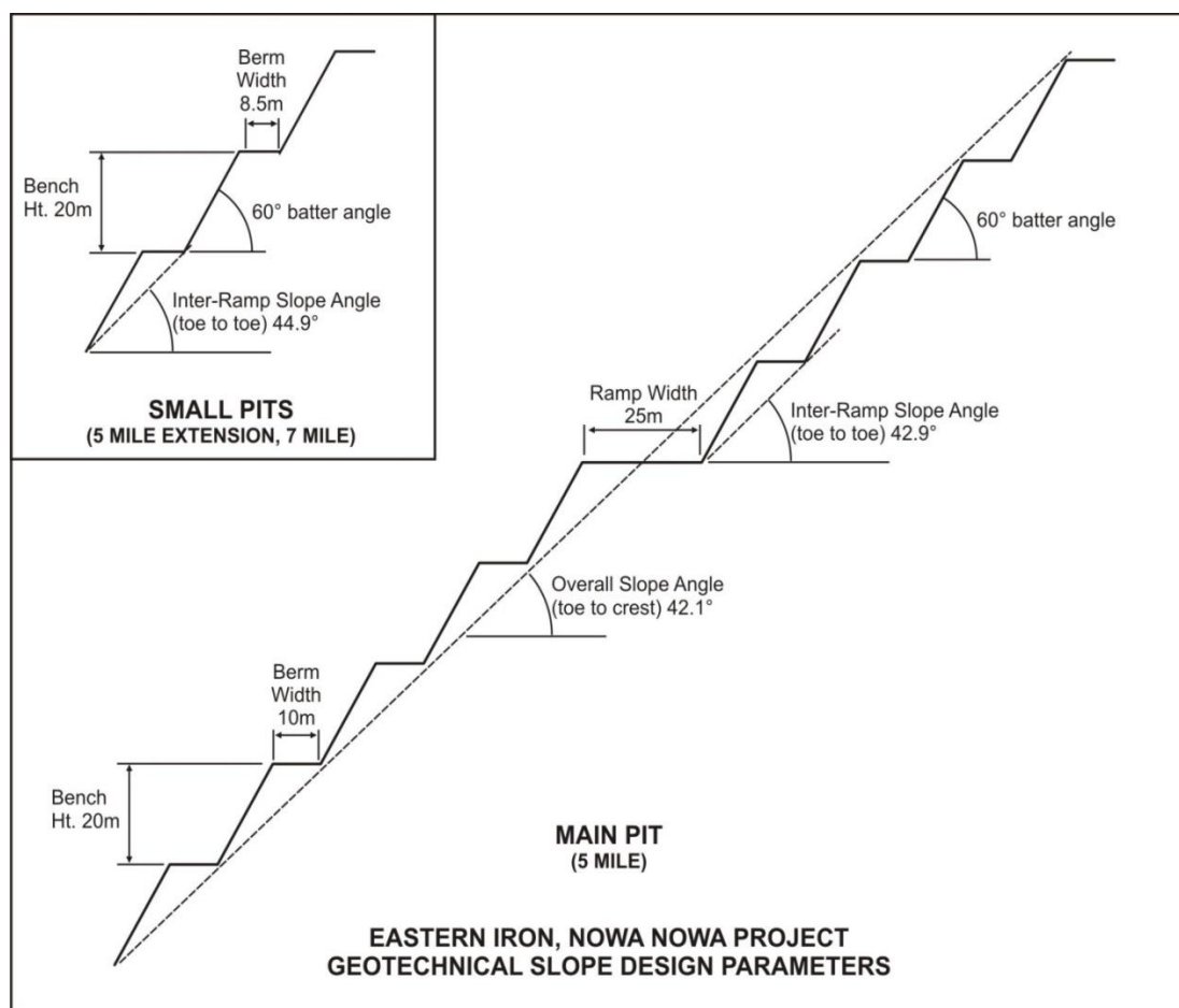
Figure 5 – Geotechnical Slope Design Parameters
