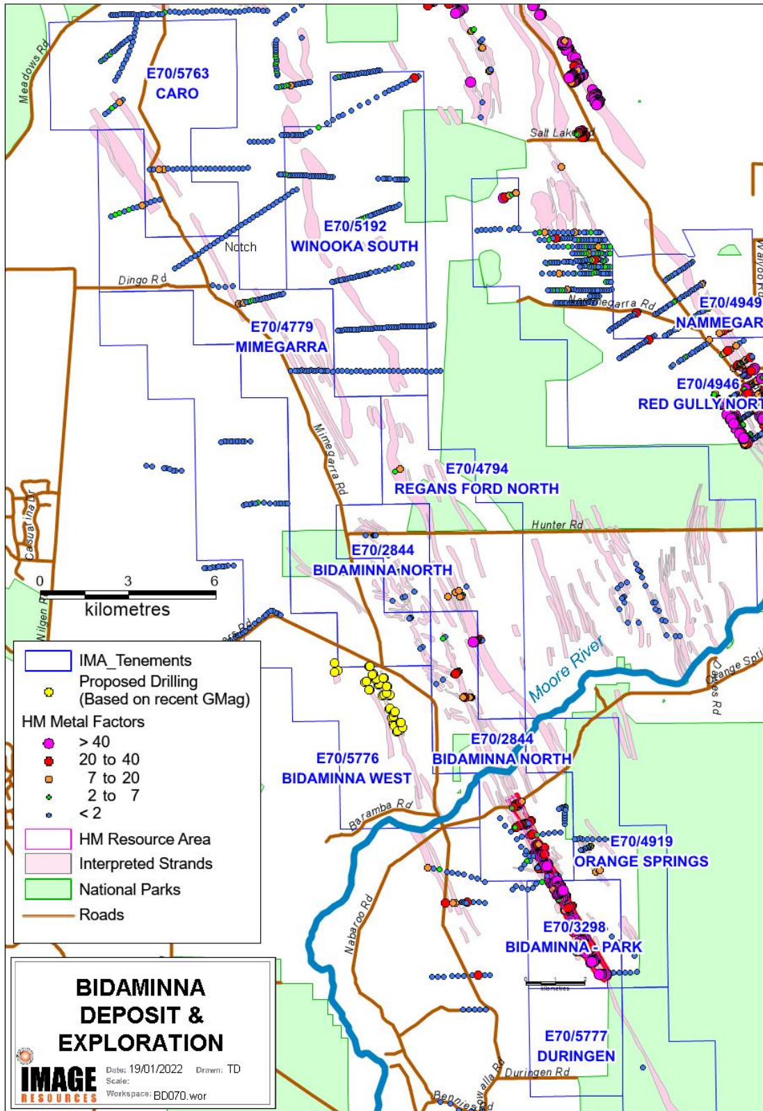
Figure 8: Drilling planned at Bidamina West shown in yellow
