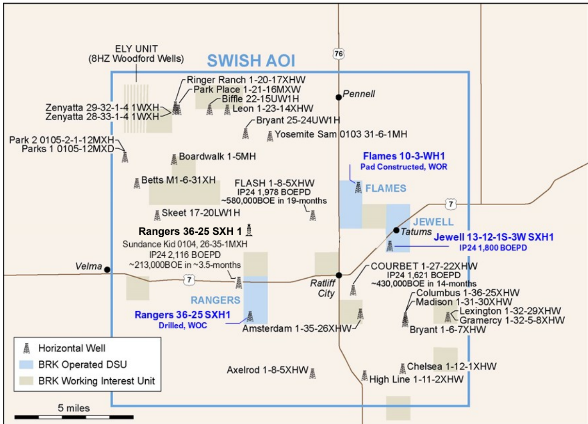
Figure 3. Location map showing the location of the Rangers Well and Brookside's three operated SWISH AOI DSU's
