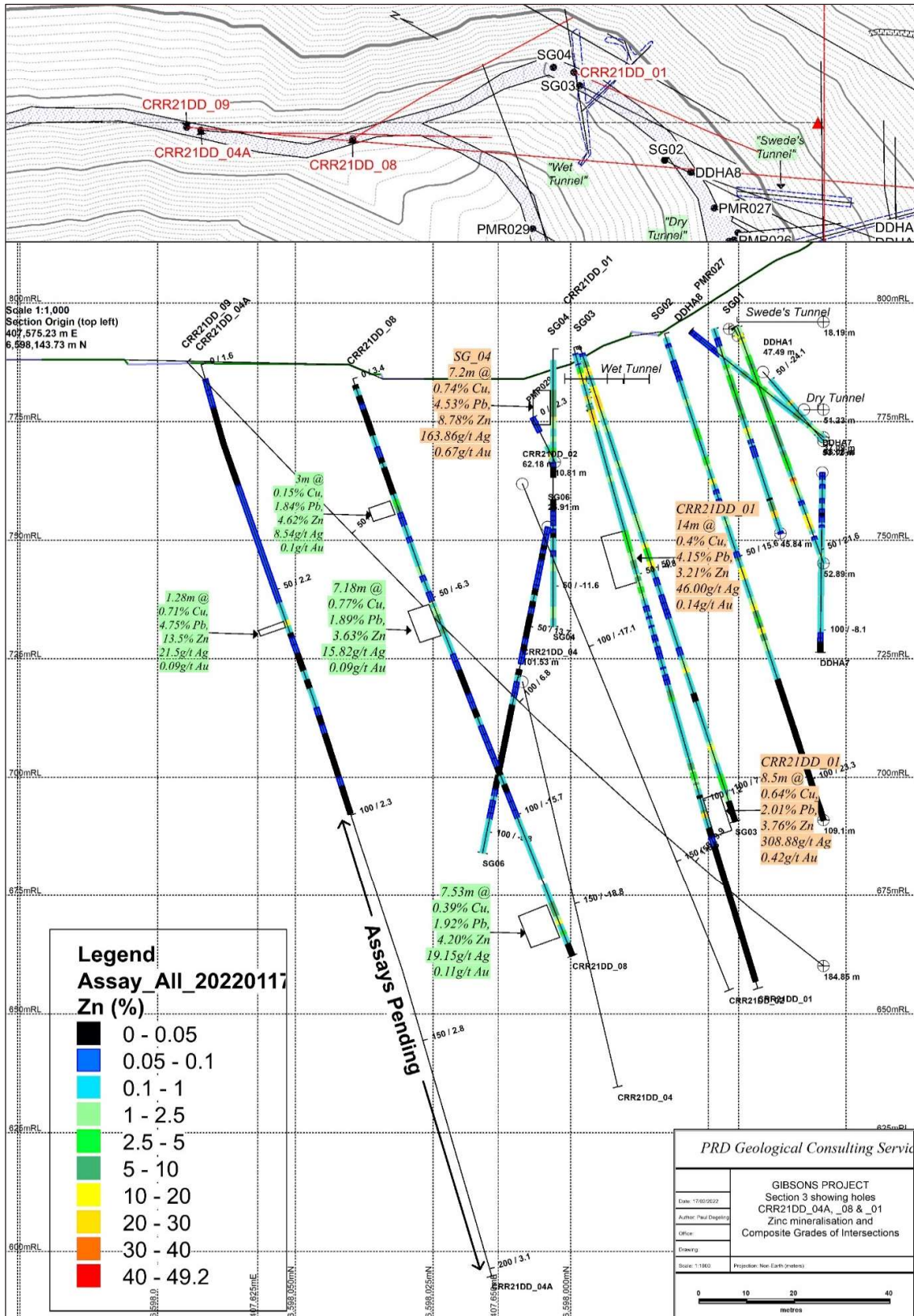
Figure 4: Cross-section and some downhole intersection, diamond drill holes CRR21DD_04A and CRR21DD_08
