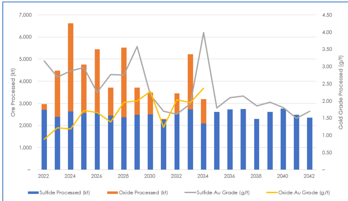
Figure 22.2 CDM21TR Reserve Case Processing
