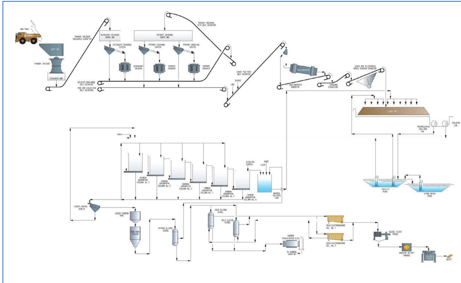
Figure 17.5 Heap Leach Process Flow Sheet
