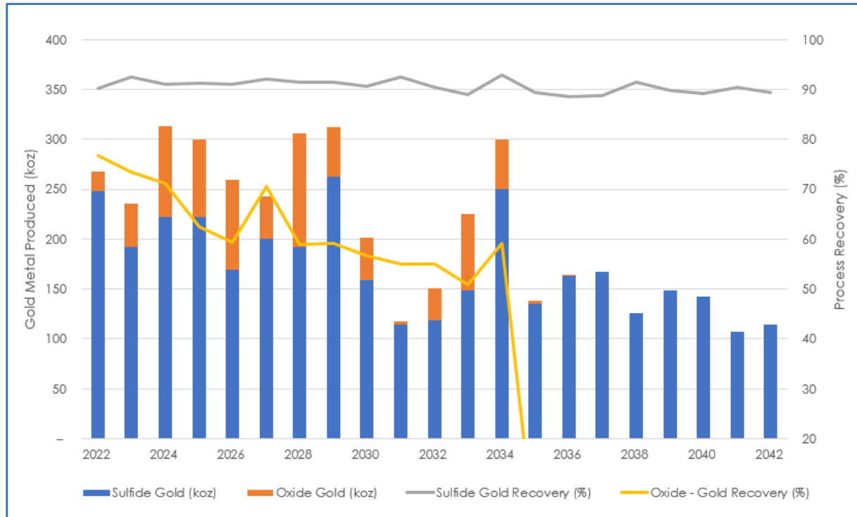
Figure 22.3 CDMP21TR Reserve Case Gold Production and Recovery
