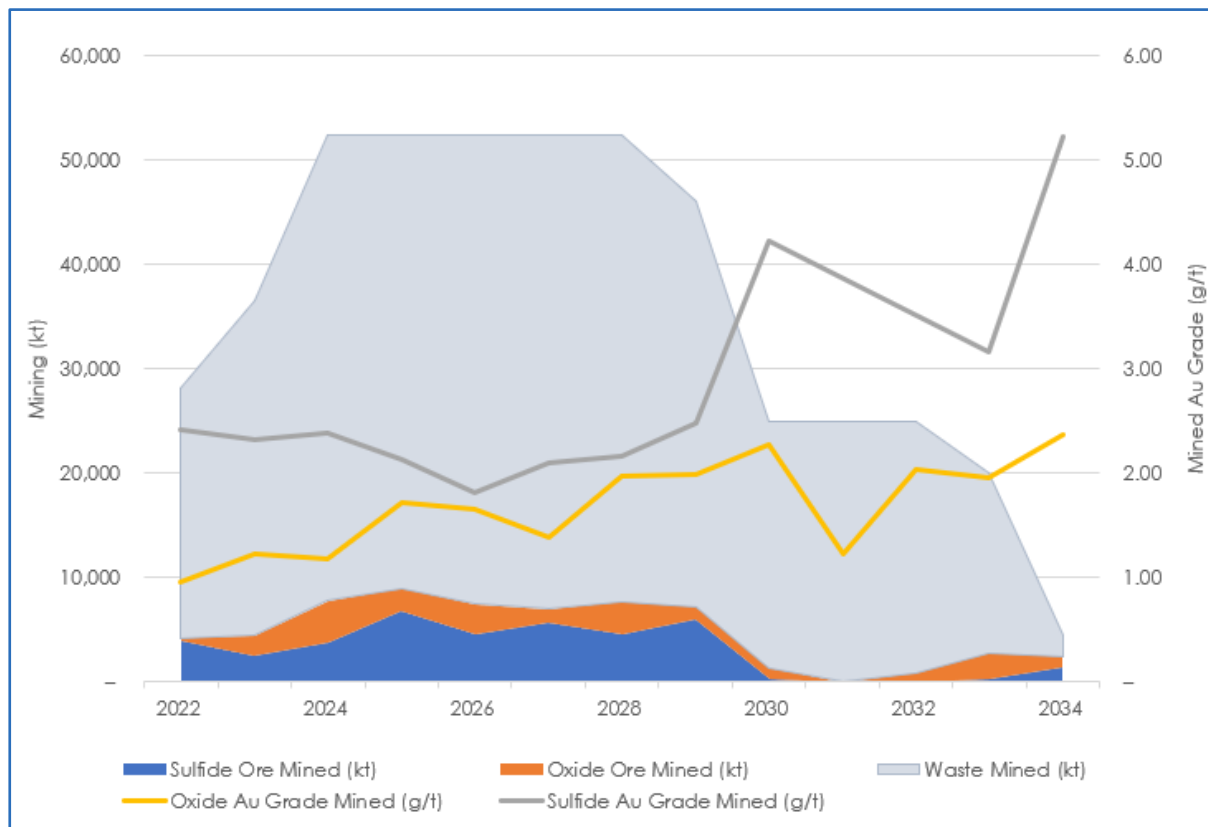
Figure 16.9 CDMP21TR Reserve Case Mining Production
