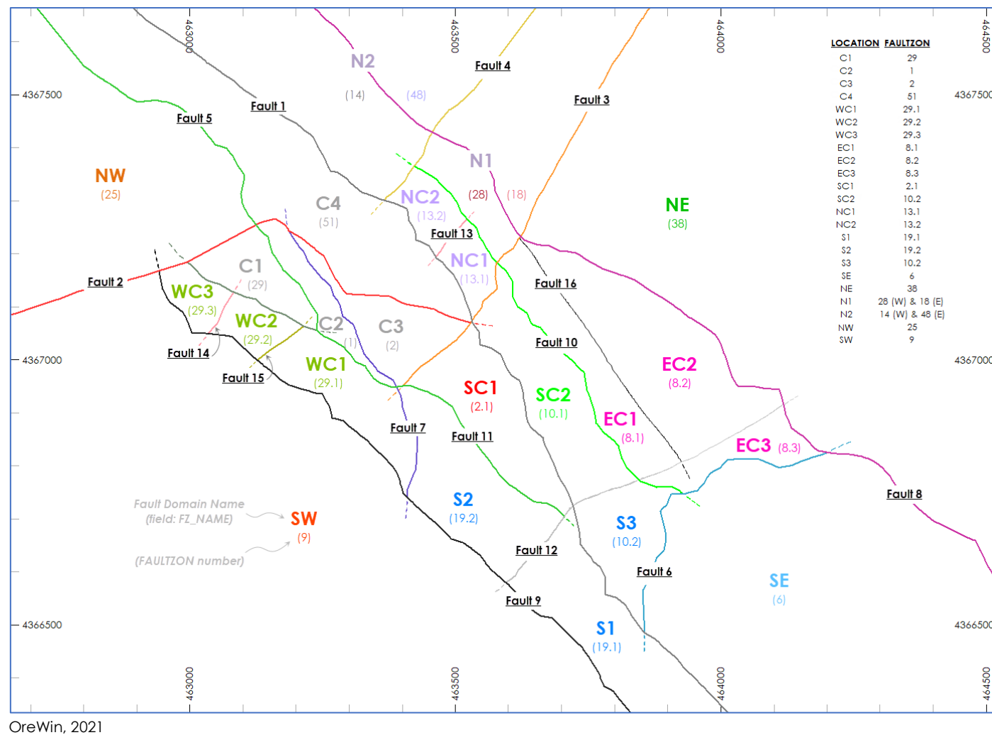
Figure 14.7 Ardich Structural Framework: Interpreted Faults and Resultant FAULTZONS
