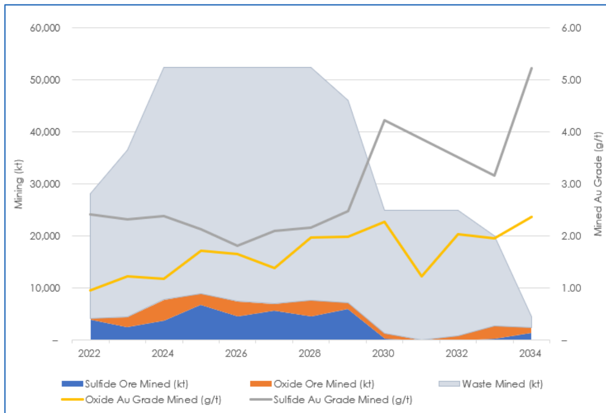
Figure 1.5 CDM21TR Reserve Case Mining Production
