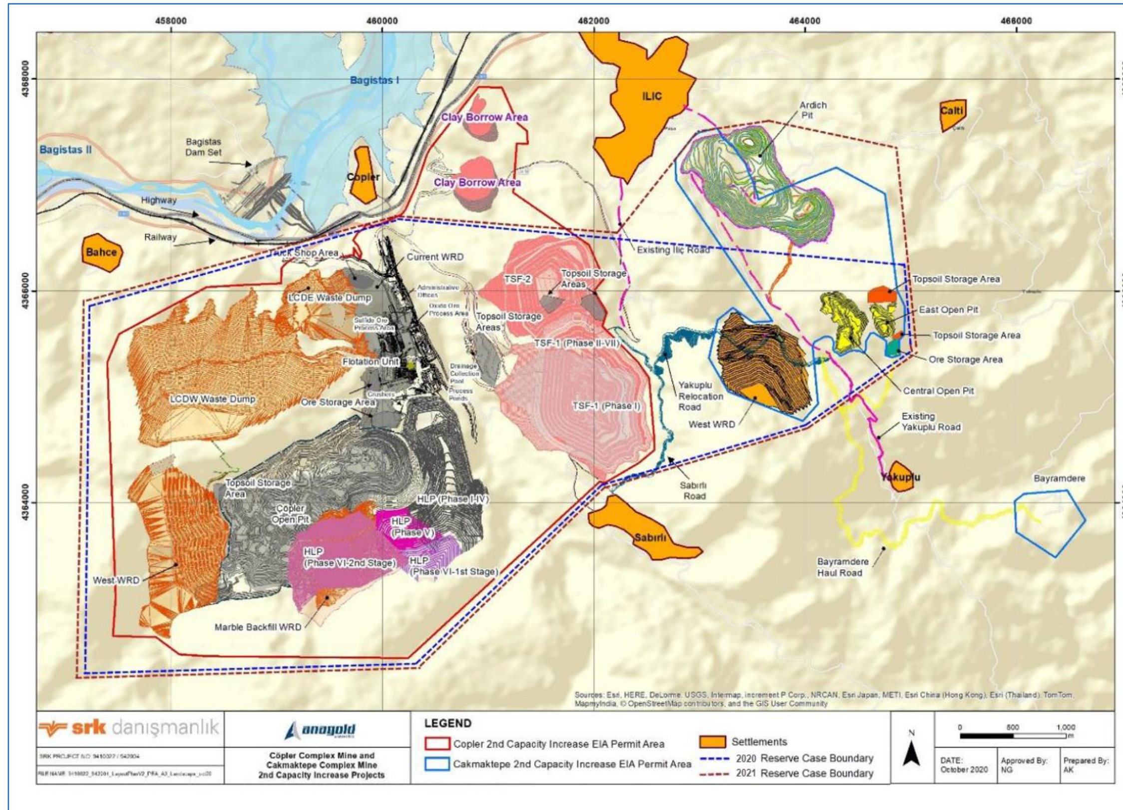
Figure 16.8 CDM21TR Reserve Case Site Plan
