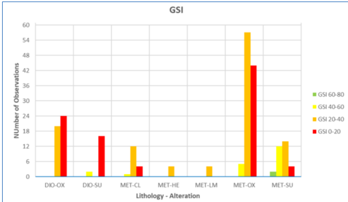
Figure 16.2 Rock Mass Quality Mapping of Main Pit
