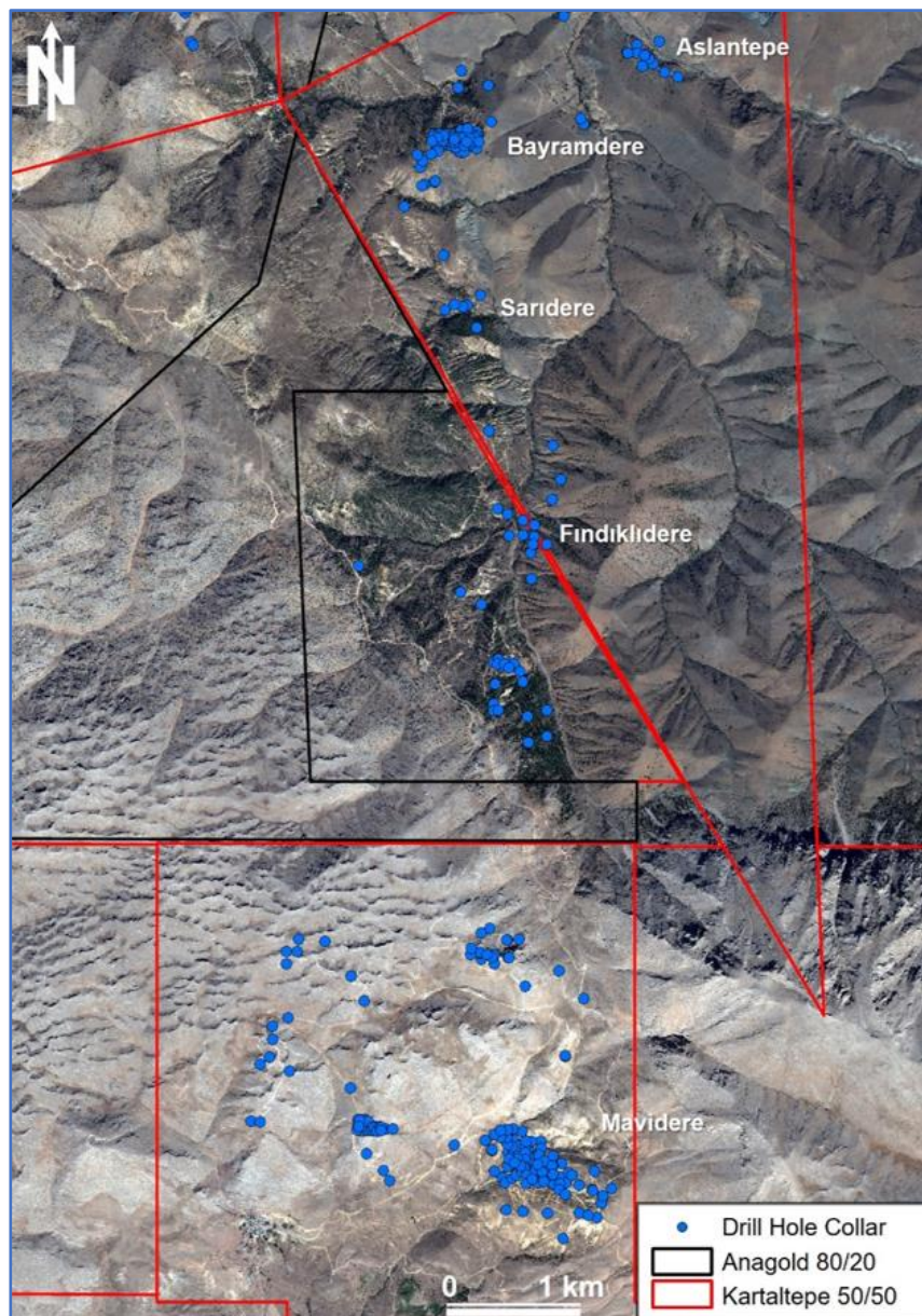
Figure 10.4 Drillhole Collar Location Plan – Maviadltin Porphyry Belt Prospects
