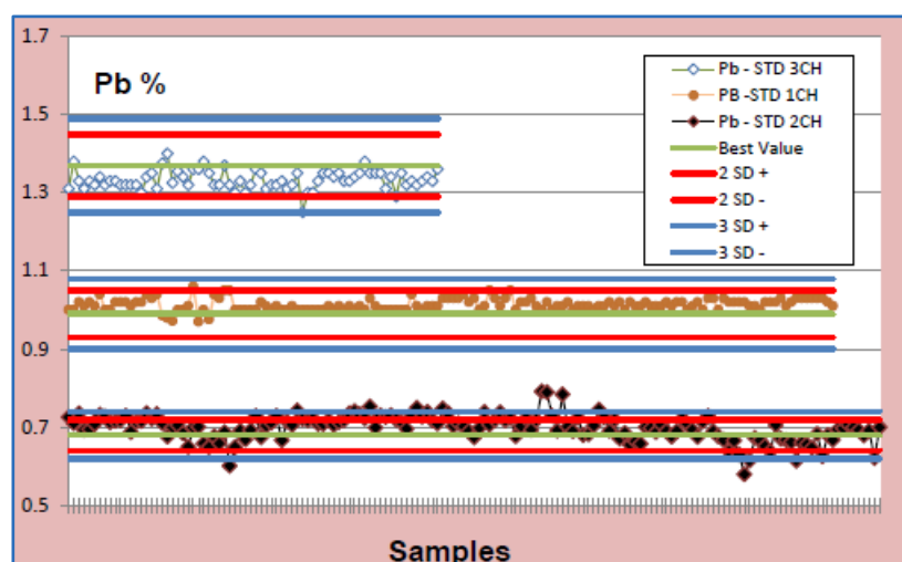
Figure 11.4 Pb Values from CRM 1-CH, 2-CH and 3-CH – Chinchillas
