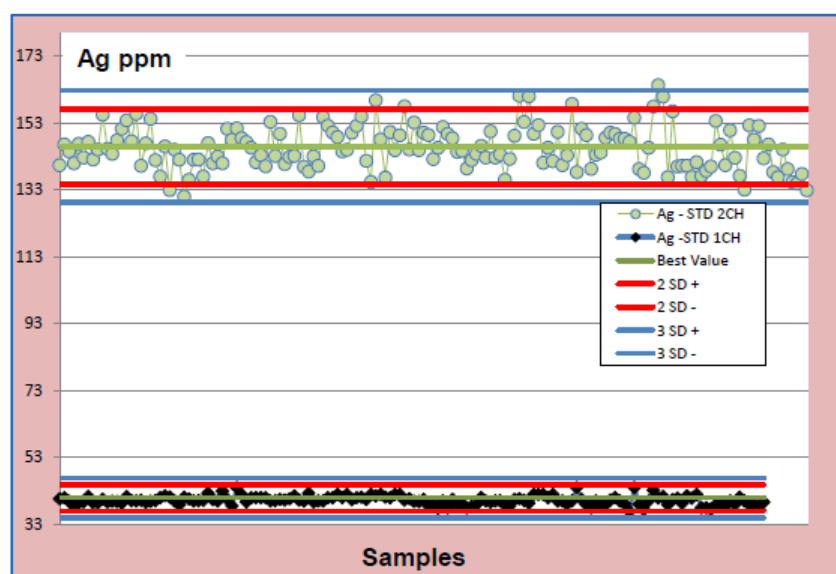
Figure 11.2 Ag Values from CRM 1-CH and 2-CH – Chinchillas
