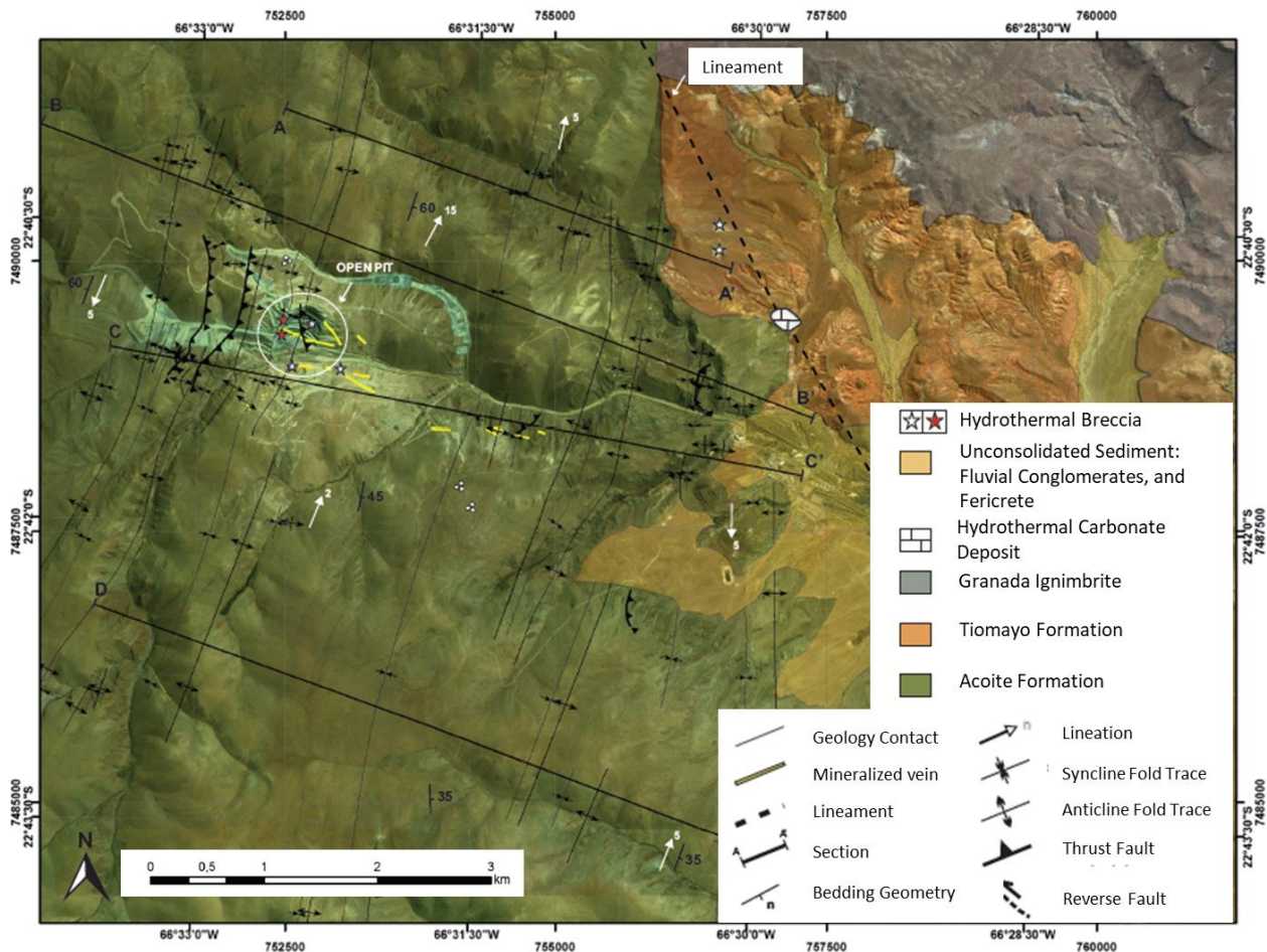
Figure 7.10 Piriquitas Geology Map
