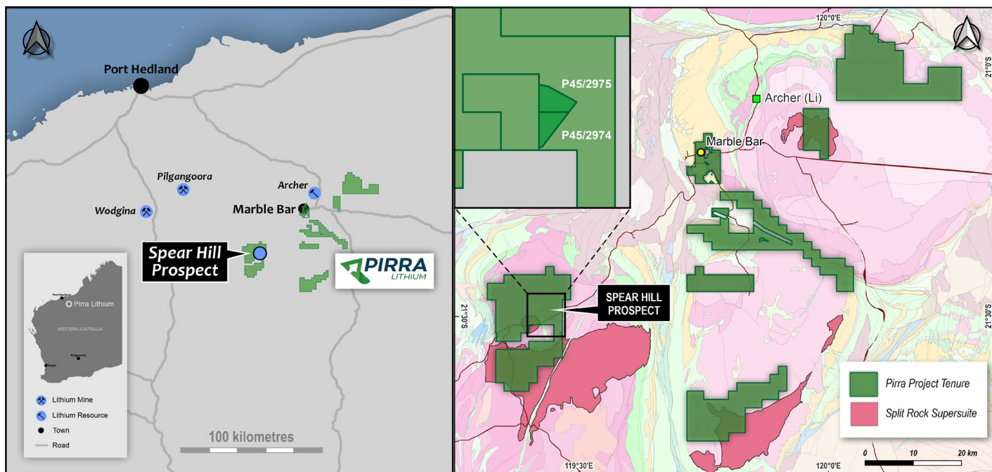
Figure 1 – Location of the Spear Hill area and tenement holdings and lithium rights of Pirra Lithium on a background of GSWA’s 1:500,000 state bedrock geology and linear structures layers.
