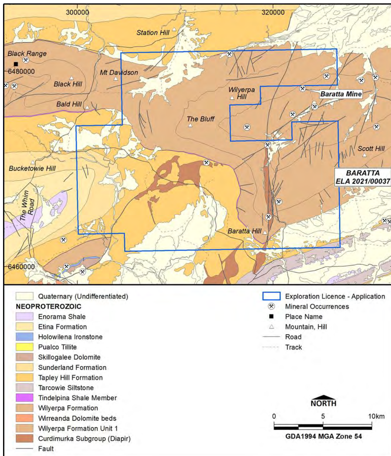
Figure 44 Baratta Project – geological map Data source: SARIG
