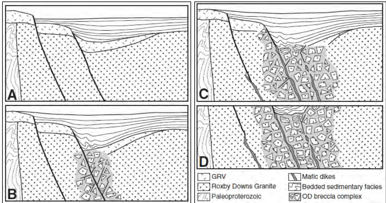
Figure 7: Model for the development of the Olympic Dam deposit
