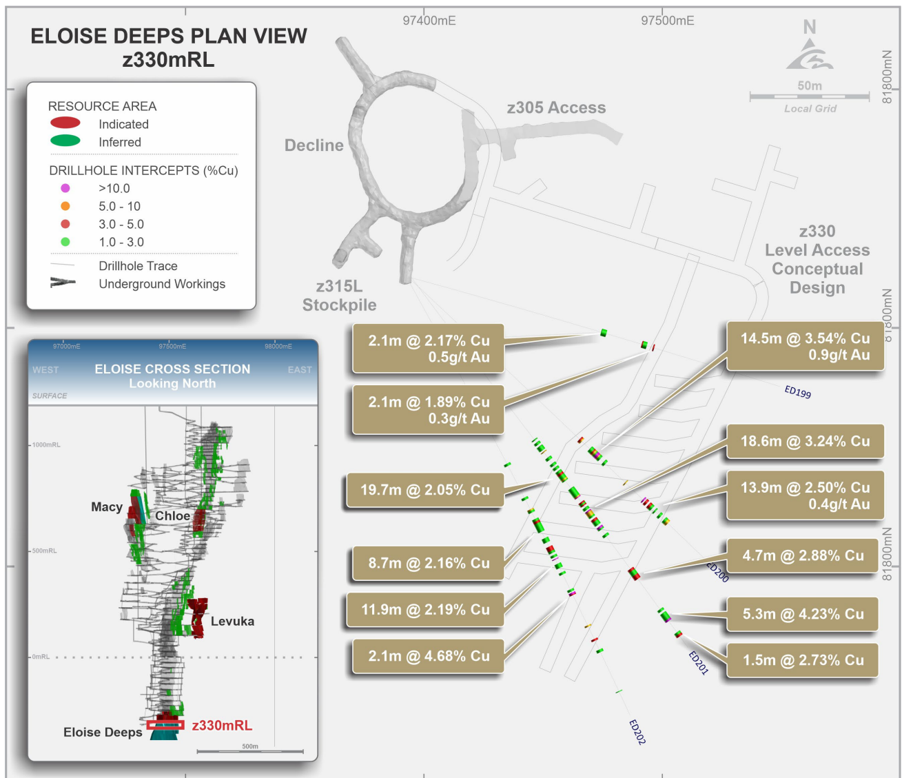
Figure 1. Plan view of Deeps drilling, sliced at z330m Level ( \pm 15 m). All intercept widths are reported as estimated true widths.
