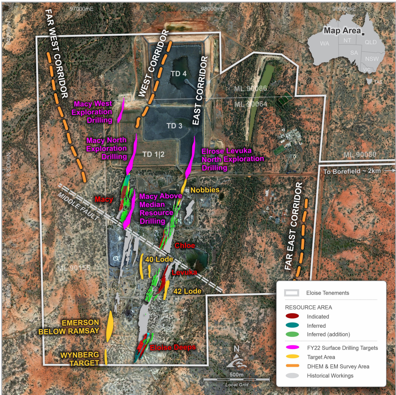
Figure 3. Location of target areas to be tested by surface drilling
