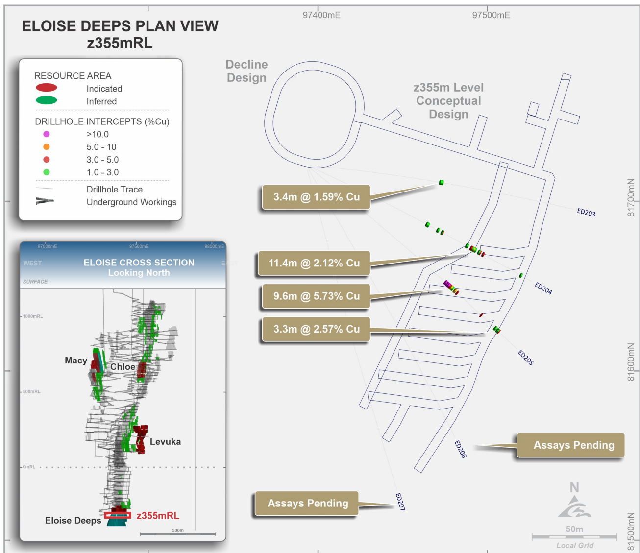
Figure 2. Plan view of Deeps drilling, sliced at z355m Level ( \pm 15 m). All intercept widths are reported as estimated true widths.
