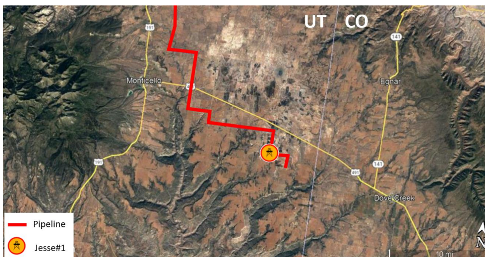
Figure 2: Jesse#1 drill site location with local pipelines
