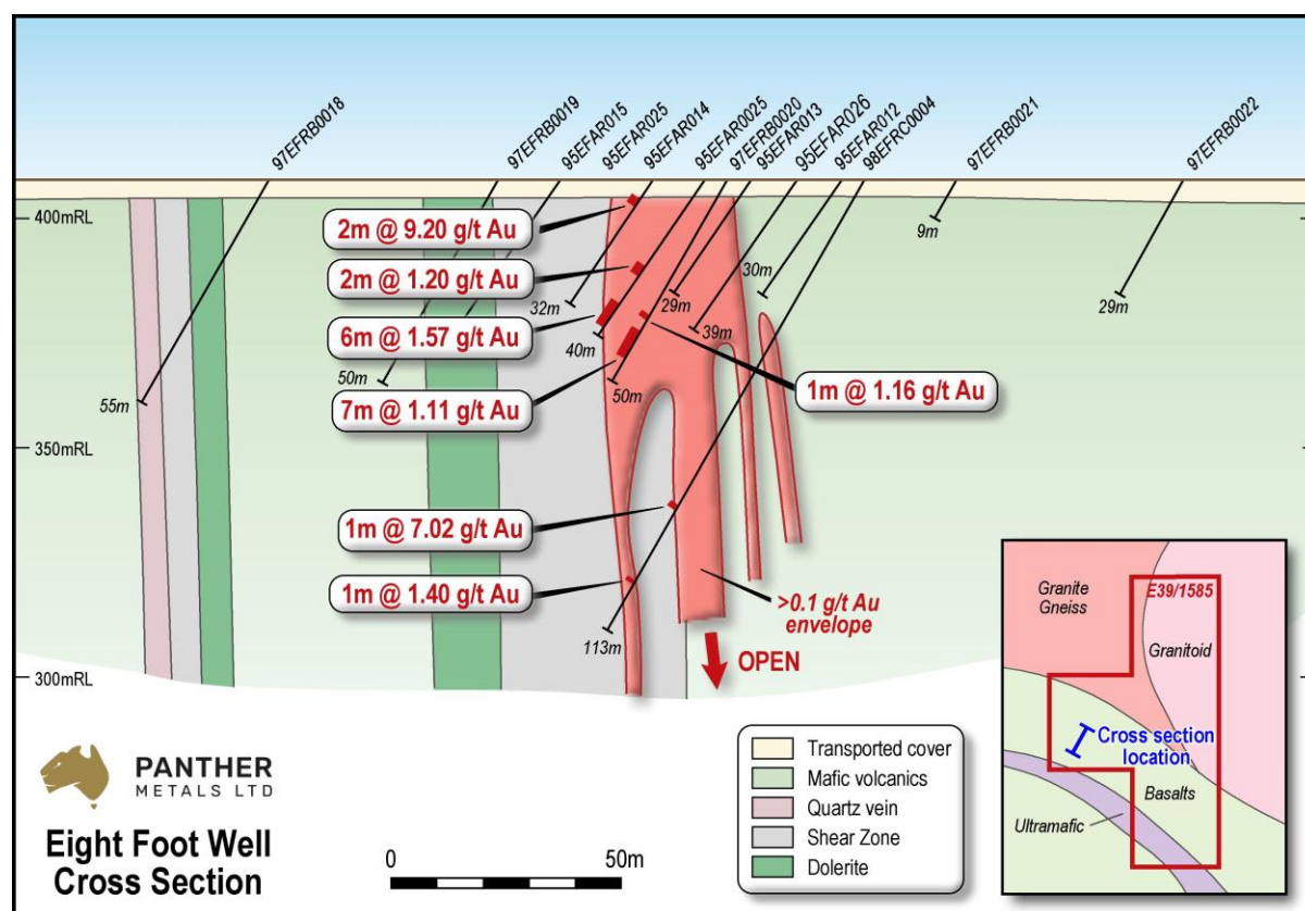
Figure 1: A cross section of the historic drilling at the Eight Foot Well gold prospect (Source: Panther Metals Prospectus)
