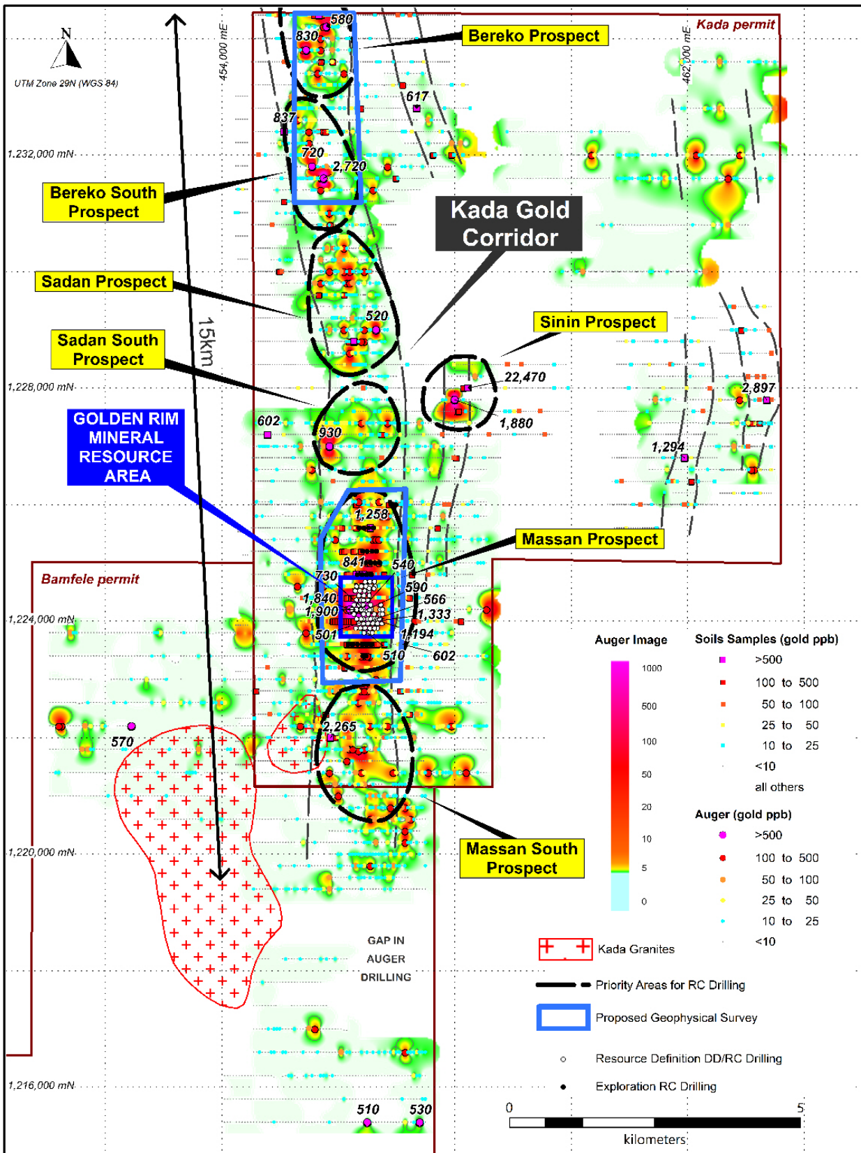
Figure 1: Imaged auger gold results highlighting the Kada Gold Corridor, with the geophysical survey areas (blue outlines).
