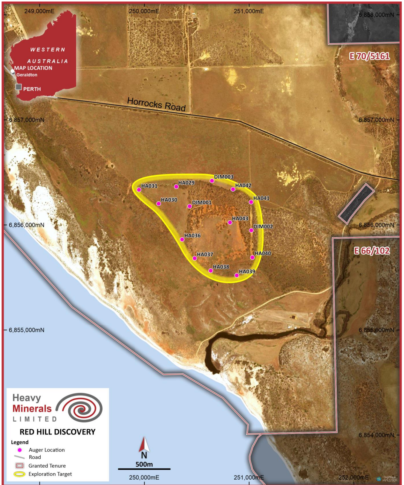
Figure 2: Auger collars referenced in this announcement
