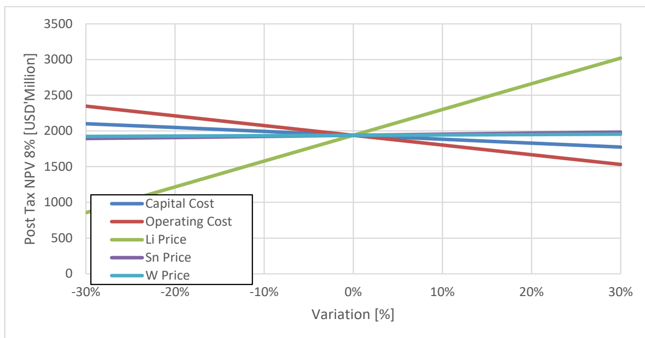
Figure 1: Sensitivity Analysis
