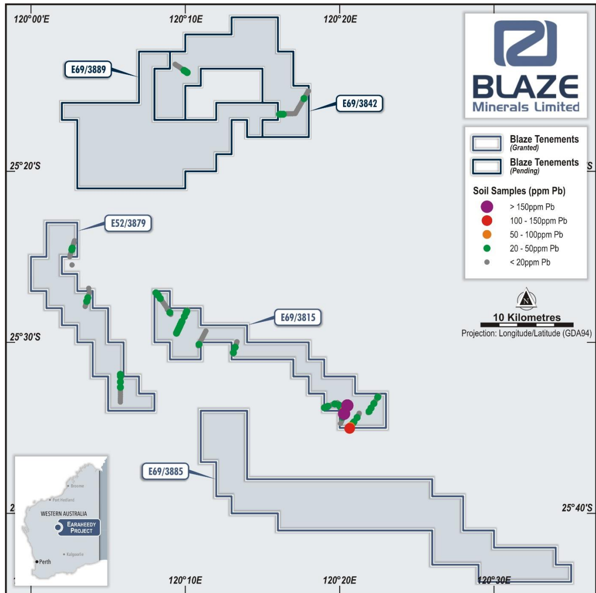
Figure 3: Blaze Soil Results (Pb)
