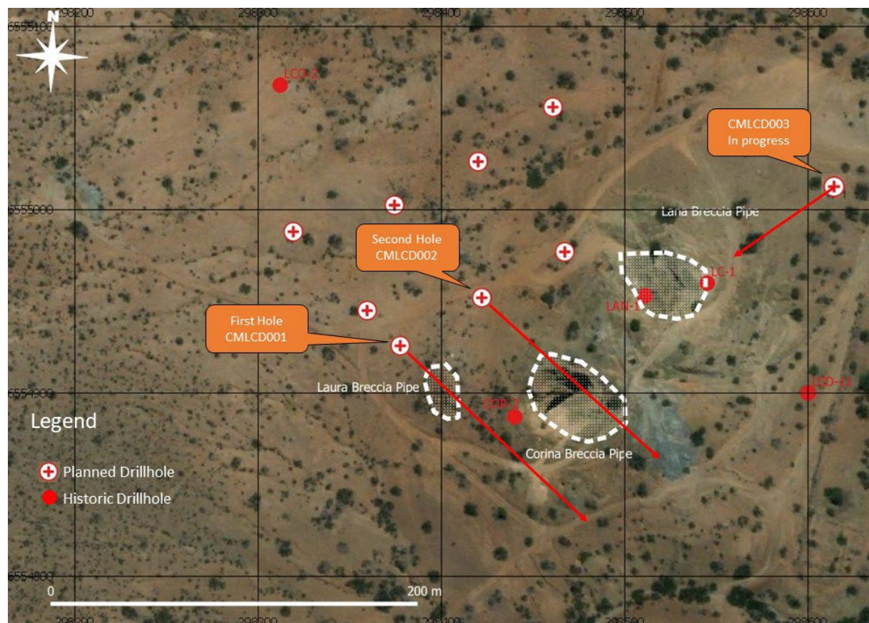
Figure 3: Plan view of drilling program collars, showing position of CMLCD001, CMLCD002, CMLCD003 and targeted breccia units.
