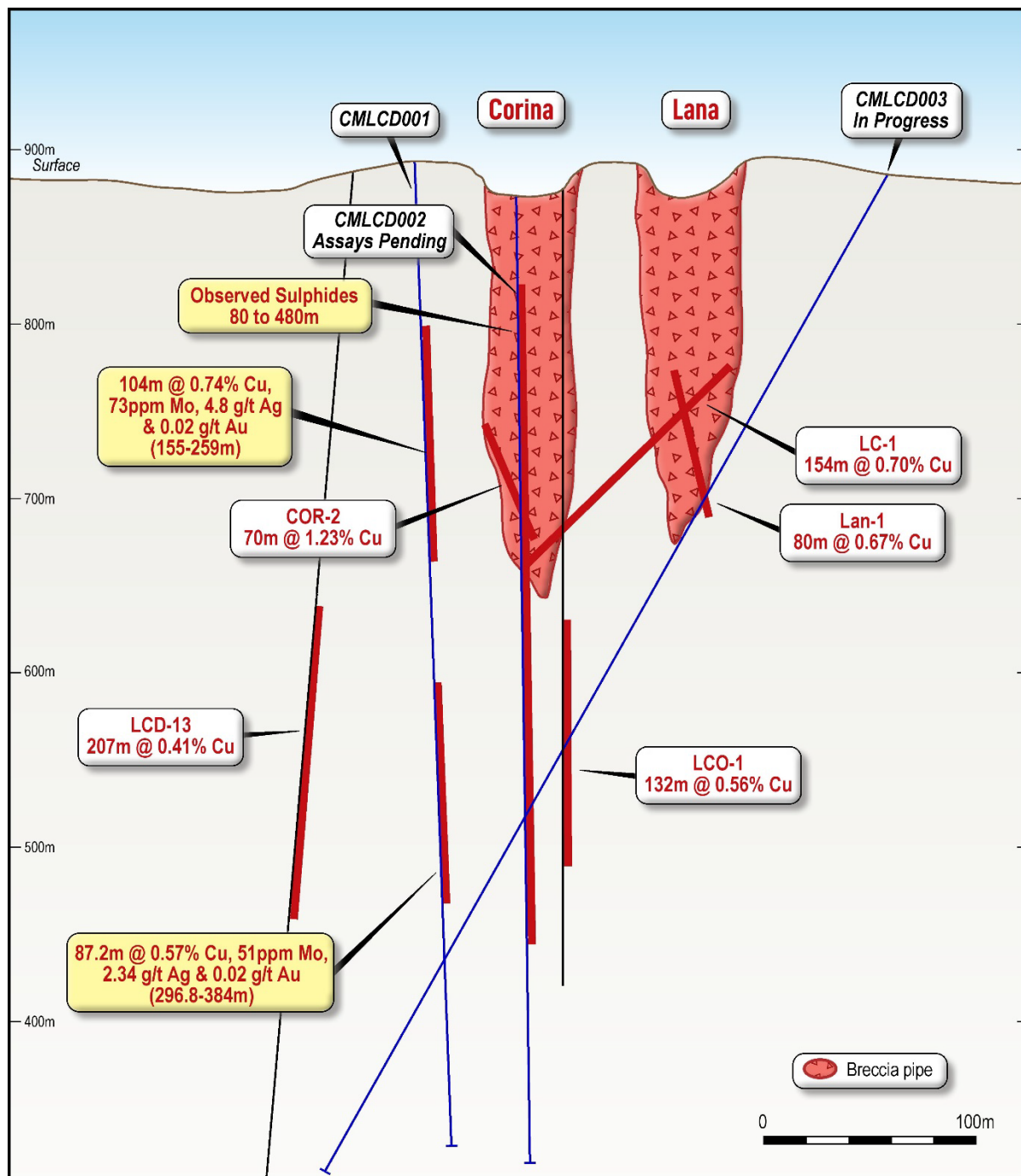
Figure 4: Long section view, looking west, showing position of CMLCD001, CMLCD002, CMLCD003 and targeted breccia units. Results for CMLDC002 are based on visual inspection only and have not been assayed.
